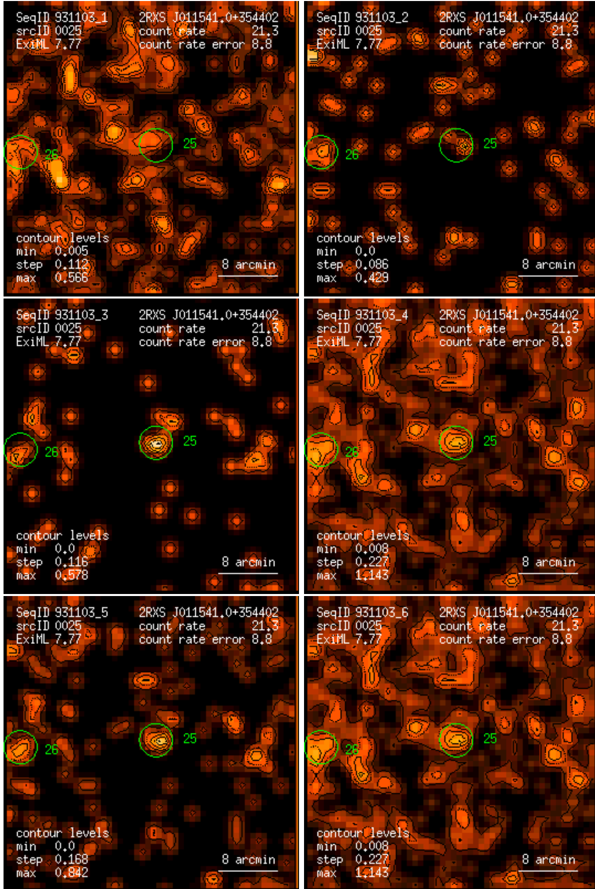
Figure 25: RASS 931103: detection 0025: band rate images, Gaussian filter: (1) PSPC channels 11 – 41, (2) 52 – 90, (3) 91 – 201, (4) 11 – 235, (5) 52 – 201, (6) 11 – 201. Broad band rates in counts/ks. Band rate contour levels in counts/ks/arcmin 2 .
