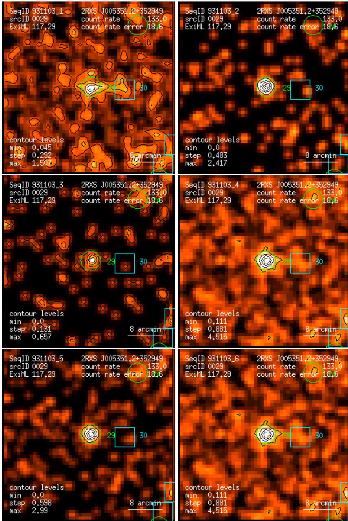
Figure 29: RASS 931103: detection 0029: band rate images, Gaussian filter: (1) PSPC channels 11 – 41, (2) 52 – 90, (3) 91 – 201, (4) 11 – 235, (5) 52 – 201, (6) 11 – 201. Broad band rates in counts/ks. Band rate contour levels in counts/ks/arcmin 2 .
