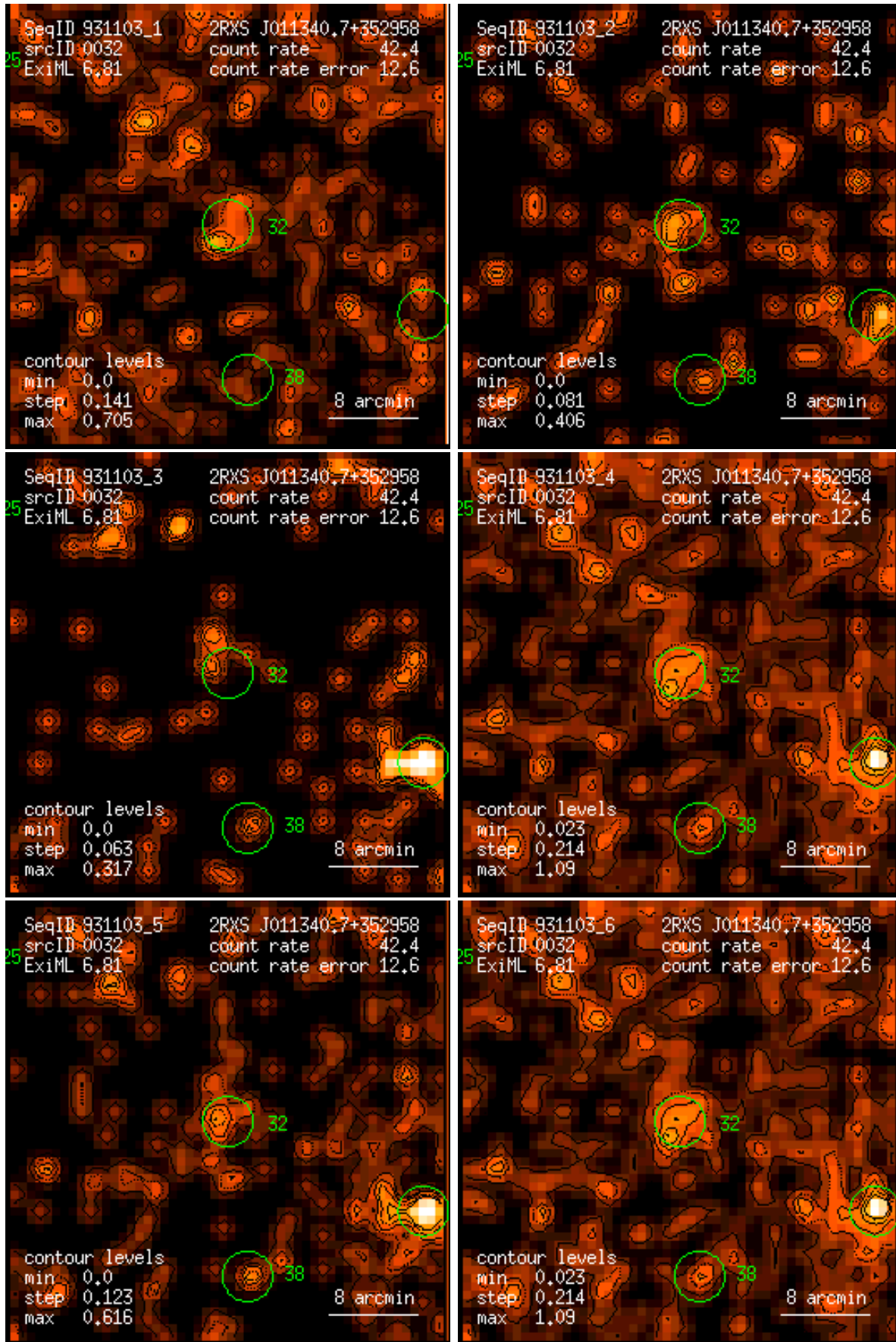
Figure 32: RASS 931103: detection 0032: band rate images, Gaussian filter: (1) PSPC channels 11 – 41, (2) 52 – 90, (3) 91 – 201, (4) 11 – 235, (5) 52 – 201, (6) 11 – 201. Broad band rates in counts/ks. Band rate contour levels in counts/ks/arcmin 2 .
