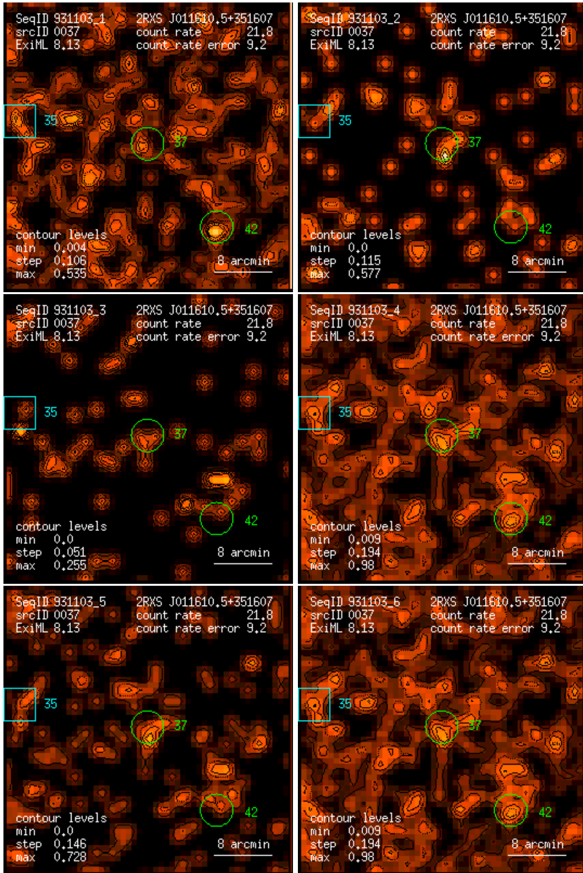
Figure 37: RASS 931103: detection 0037: band rate images, Gaussian filter: (1) PSPC channels 11 – 41, (2) 52 – 90, (3) 91 – 201, (4) 11 – 235, (5) 52 – 201, (6) 11 – 201. Broad band rates in counts/ks. Band rate contour levels in counts/ks/arcmin 2 .
