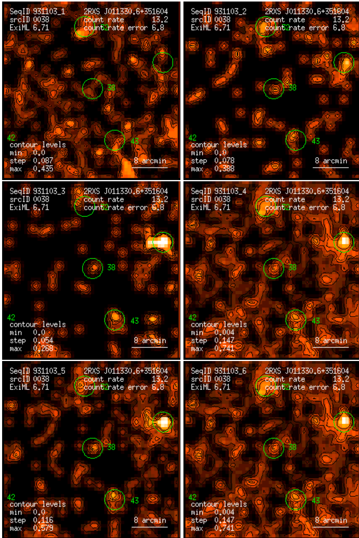
Figure 38: RASS 931103: detection 0038: band rate images, Gaussian filter: (1) PSPC channels 11 – 41, (2) 52 – 90, (3) 91 – 201, (4) 11 – 235, (5) 52 – 201, (6) 11 – 201. Broad band rates in counts/ks. Band rate contour levels in counts/ks/arcmin 2 .
