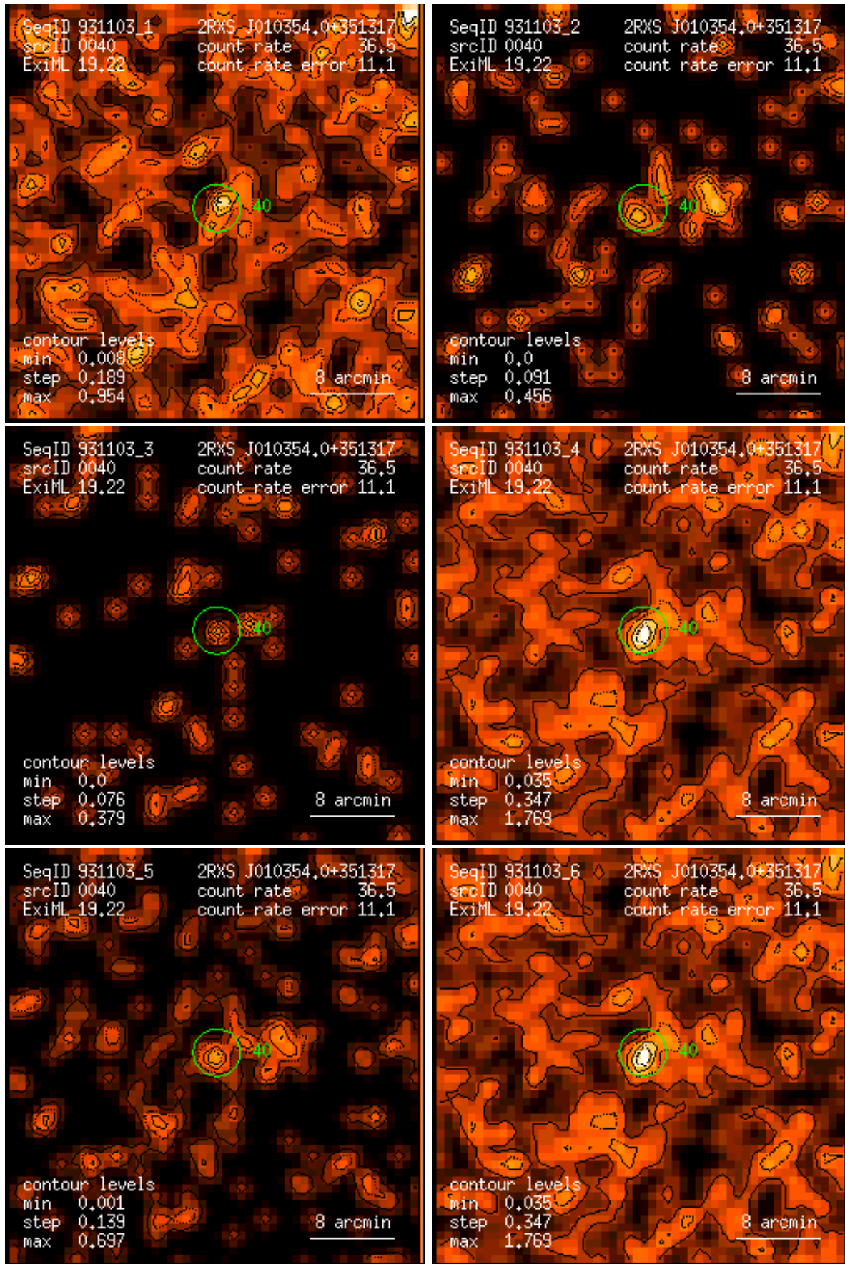
Figure 40: RASS 931103: detection 0040: band rate images, Gaussian filter: (1) PSPC channels 11 – 41, (2) 52 – 90, (3) 91 – 201, (4) 11 – 235, (5) 52 – 201, (6) 11 – 201. Broad band rates in counts/ks. Band rate contour levels in counts/ks/arcmin 2 .
