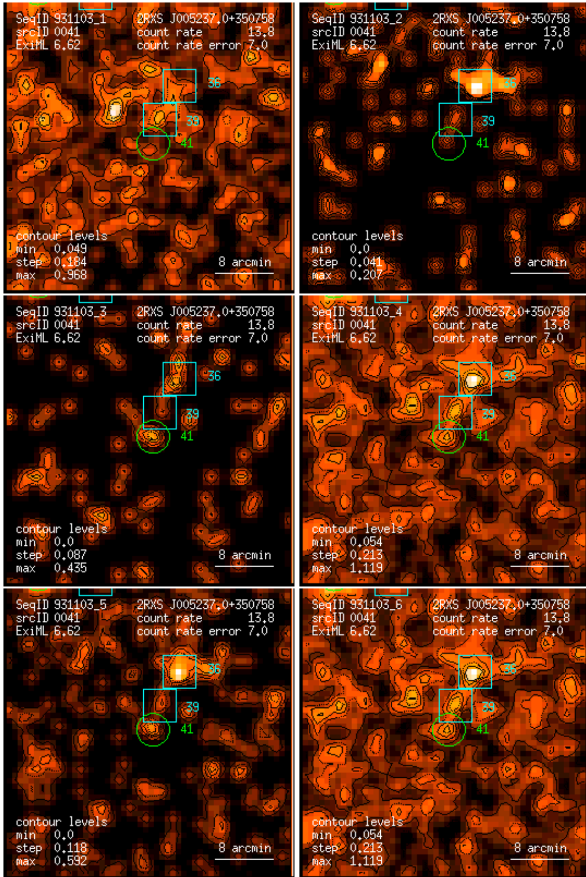
Figure 41: RASS 931103: detection 0041: band rate images, Gaussian filter: (1) PSPC channels 11 – 41, (2) 52 – 90, (3) 91 – 201, (4) 11 – 235, (5) 52 – 201, (6) 11 – 201. Broad band rates in counts/ks. Band rate contour levels in counts/ks/arcmin 2 .
