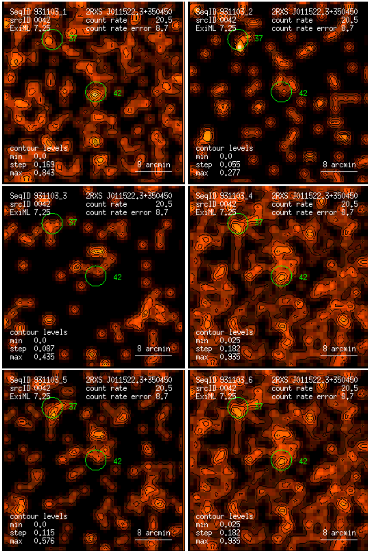
Figure 42: RASS 931103: detection 0042: band rate images, Gaussian filter: (1) PSPC channels 11 – 41, (2) 52 – 90, (3) 91 – 201, (4) 11 – 235, (5) 52 – 201, (6) 11 – 201. Broad band rates in counts/ks. Band rate contour levels in counts/ks/arcmin 2 .
