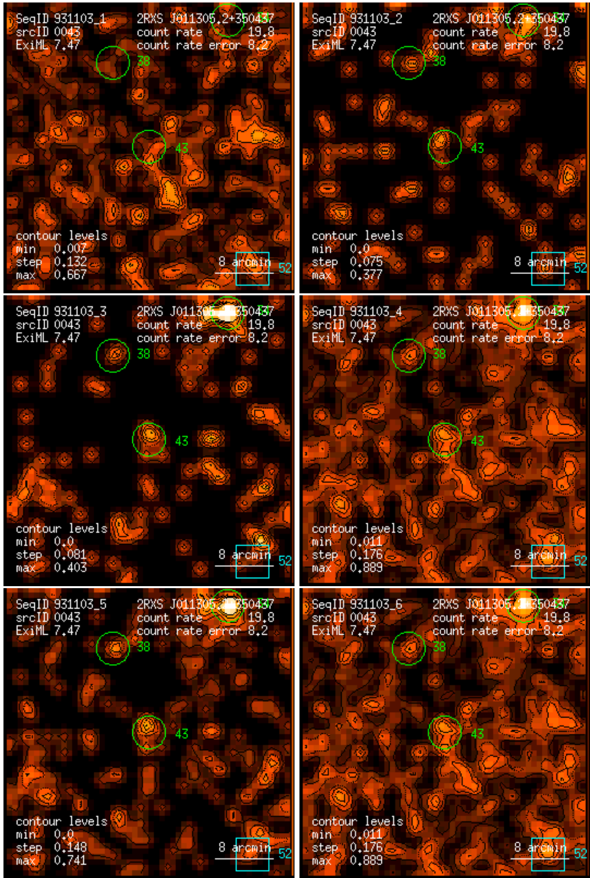
Figure 43: RASS 931103: detection 0043: band rate images, Gaussian filter: (1) PSPC channels 11 – 41, (2) 52 – 90, (3) 91 – 201, (4) 11 – 235, (5) 52 – 201, (6) 11 – 201. Broad band rates in counts/ks. Band rate contour levels in counts/ks/arcmin 2 .
