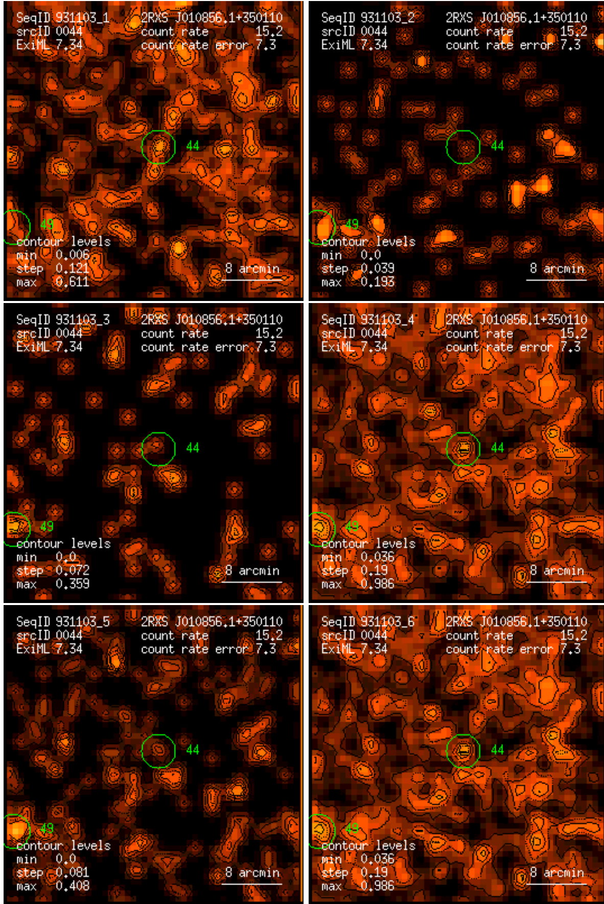
Figure 44: RASS 931103: detection 0044: band rate images, Gaussian filter: (1) PSPC channels 11 – 41, (2) 52 – 90, (3) 91 – 201, (4) 11 – 235, (5) 52 – 201, (6) 11 – 201. Broad band rates in counts/ks. Band rate contour levels in counts/ks/arcmin 2 .
