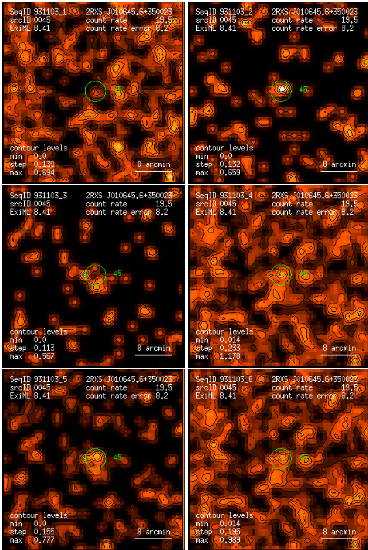
Figure 45: RASS 931103: detection 0045: band rate images, Gaussian filter: (1) PSPC channels 11 – 41, (2) 52 – 90, (3) 91 – 201, (4) 11 – 235, (5) 52 – 201, (6) 11 – 201. Broad band rates in counts/ks. Band rate contour levels in counts/ks/arcmin 2 .
