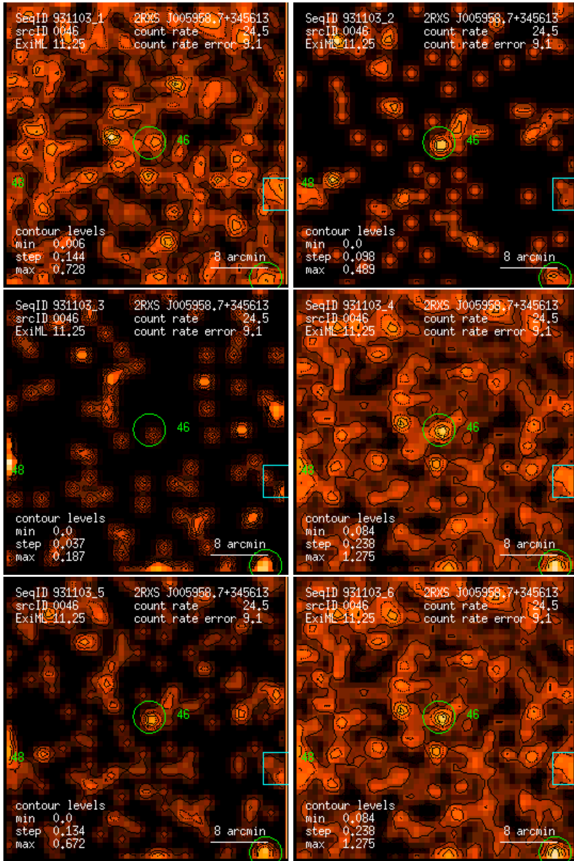
Figure 46: RASS 931103: detection 0046: band rate images, Gaussian filter: (1) PSPC channels 11 – 41, (2) 52 – 90, (3) 91 – 201, (4) 11 – 235, (5) 52 – 201, (6) 11 – 201. Broad band rates in counts/ks. Band rate contour levels in counts/ks/arcmin 2 .
