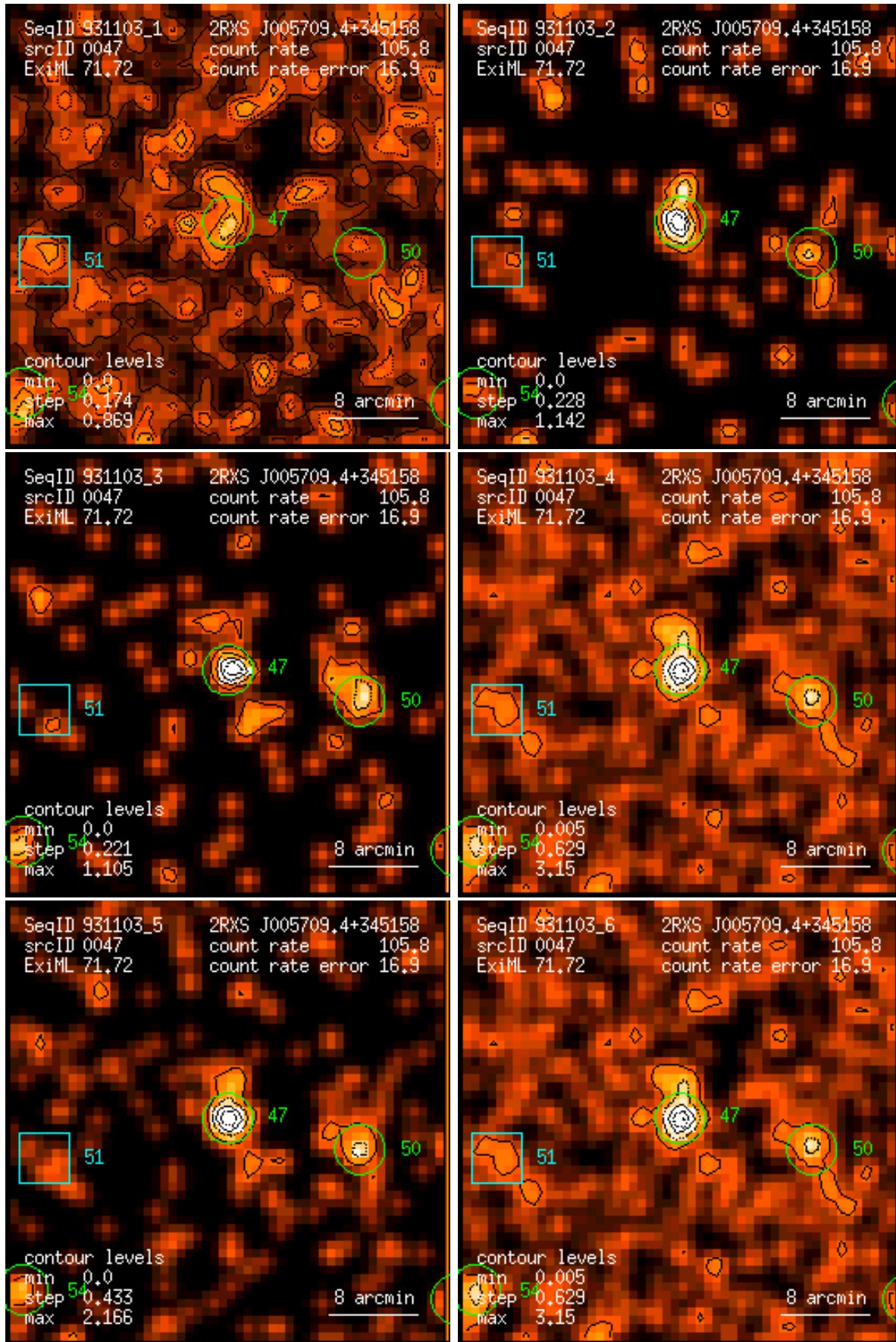
Figure 47: RASS 931103: detection 0047: band rate images, Gaussian filter: (1) PSPC channels 11 – 41, (2) 52 – 90, (3) 91 – 201, (4) 11 – 235, (5) 52 – 201, (6) 11 – 201. Broad band rates in counts/ks. Band rate contour levels in counts/ks/arcmin 2 .
