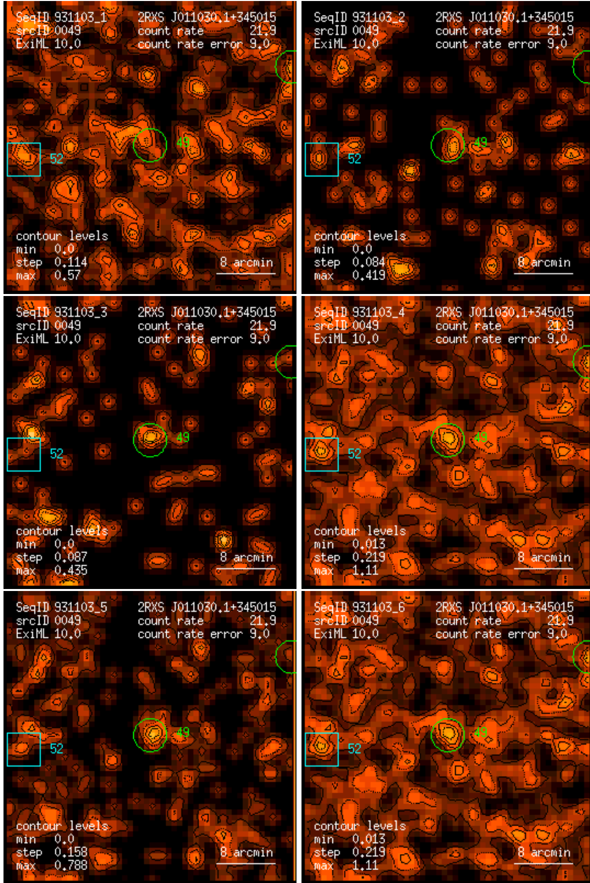
Figure 49: RASS 931103: detection 0049: band rate images, Gaussian filter: (1) PSPC channels 11 – 41, (2) 52 – 90, (3) 91 – 201, (4) 11 – 235, (5) 52 – 201, (6) 11 – 201. Broad band rates in counts/ks. Band rate contour levels in counts/ks/arcmin 2 .
