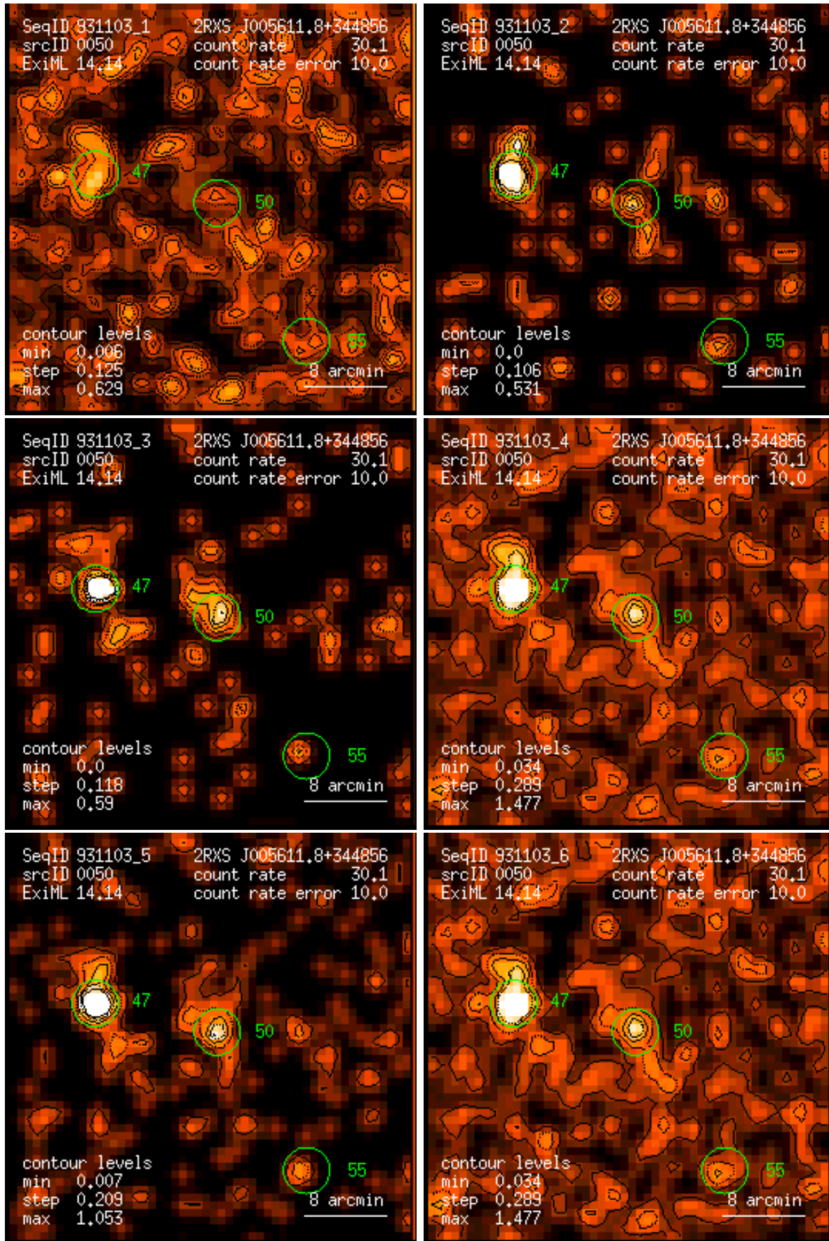
Figure 50: RASS 931103: detection 0050: band rate images, Gaussian filter: (1) PSPC channels 11 – 41, (2) 52 – 90, (3) 91 – 201, (4) 11 – 235, (5) 52 – 201, (6) 11 – 201. Broad band rates in counts/ks. Band rate contour levels in counts/ks/arcmin 2 .
