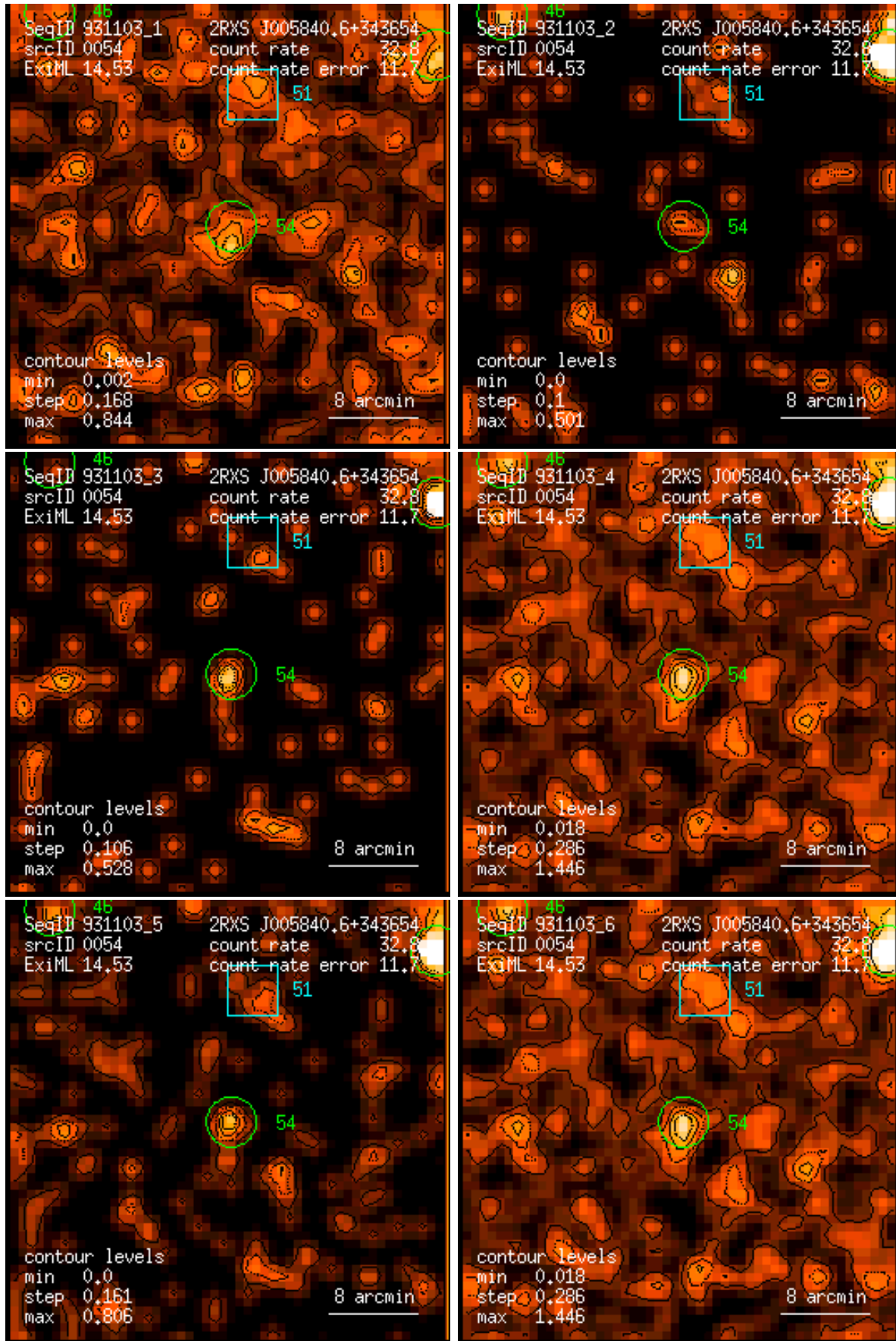
Figure 54: RASS 931103: detection 0054: band rate images, Gaussian filter: (1) PSPC channels 11 – 41, (2) 52 – 90, (3) 91 – 201, (4) 11 – 235, (5) 52 – 201, (6) 11 – 201. Broad band rates in counts/ks. Band rate contour levels in counts/ks/arcmin 2 .
