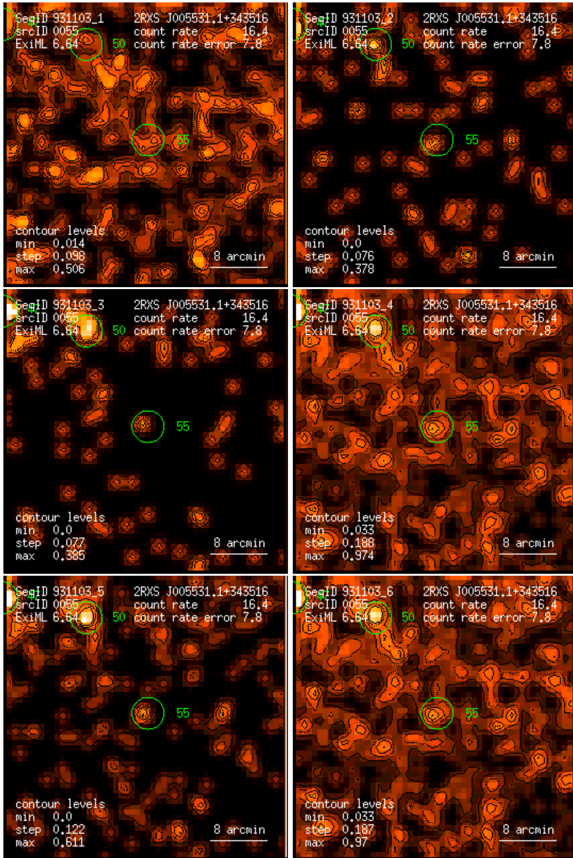
Figure 55: RASS 931103: detection 0055: band rate images, Gaussian filter: (1) PSPC channels 11 – 41, (2) 52 – 90, (3) 91 – 201, (4) 11 – 235, (5) 52 – 201, (6) 11 – 201. Broad band rates in counts/ks. Band rate contour levels in counts/ks/arcmin 2 .
