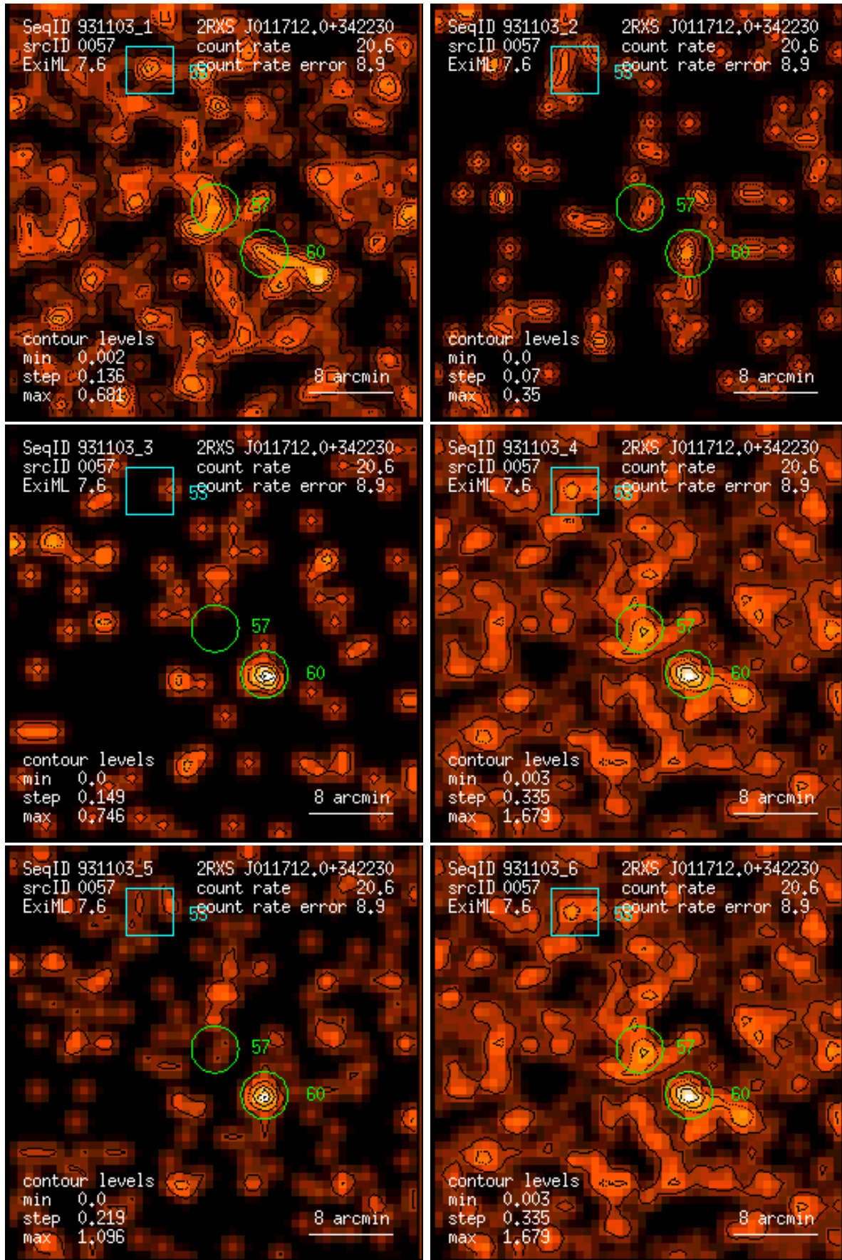
Figure 57: RASS 931103: detection 0057: band rate images, Gaussian filter: (1) PSPC channels 11 – 41, (2) 52 – 90, (3) 91 – 201, (4) 11 – 235, (5) 52 – 201, (6) 11 – 201. Broad band rates in counts/ks. Band rate contour levels in counts/ks/arcmin 2 .
