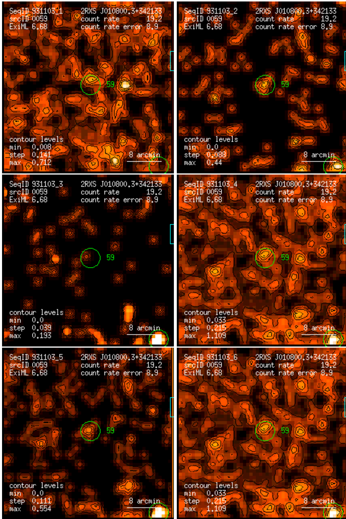
Figure 59: RASS 931103: detection 0059: band rate images, Gaussian filter: (1) PSPC channels 11 – 41, (2) 52 – 90, (3) 91 – 201, (4) 11 – 235, (5) 52 – 201, (6) 11 – 201. Broad band rates in counts/ks. Band rate contour levels in counts/ks/arcmin 2 .
