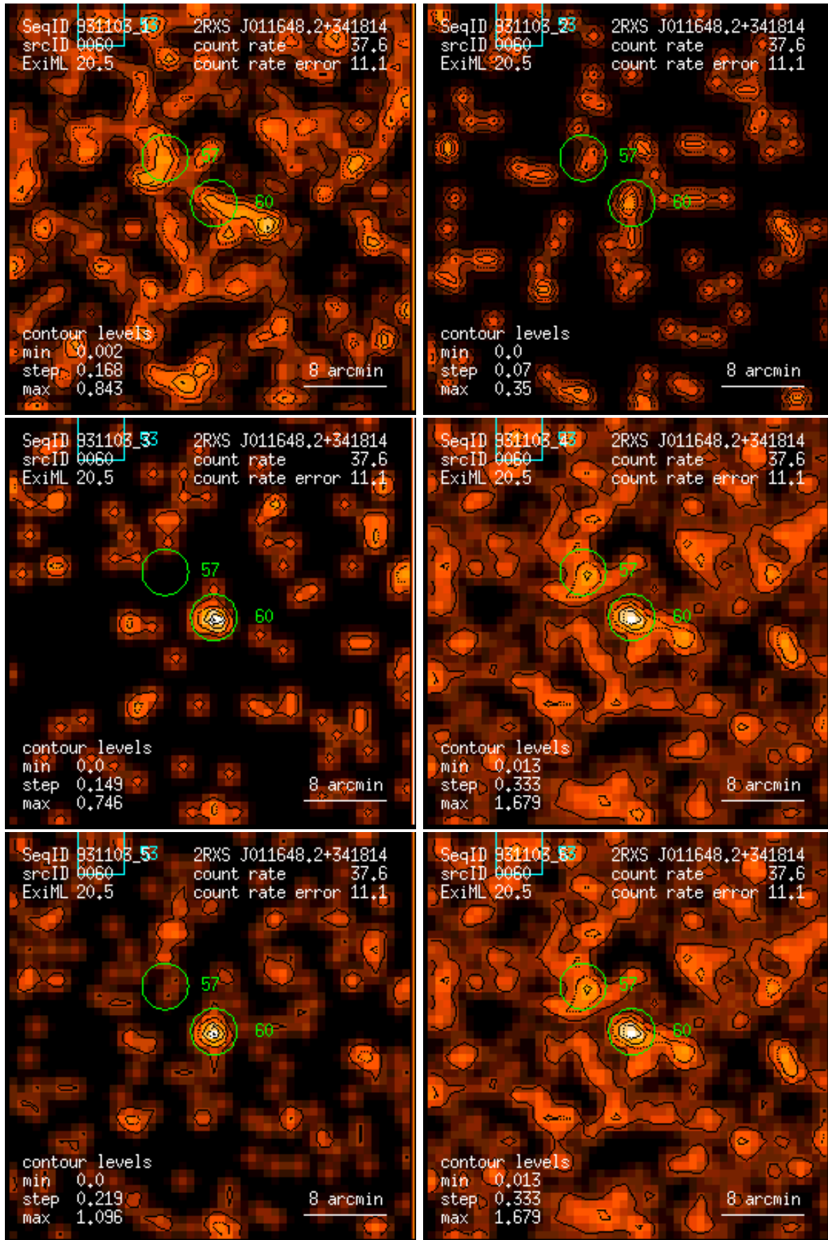
Figure 60: RASS 931103: detection 0060: band rate images, Gaussian filter: (1) PSPC channels 11 – 41, (2) 52 – 90, (3) 91 – 201, (4) 11 – 235, (5) 52 – 201, (6) 11 – 201. Broad band rates in counts/ks. Band rate contour levels in counts/ks/arcmin 2 .
