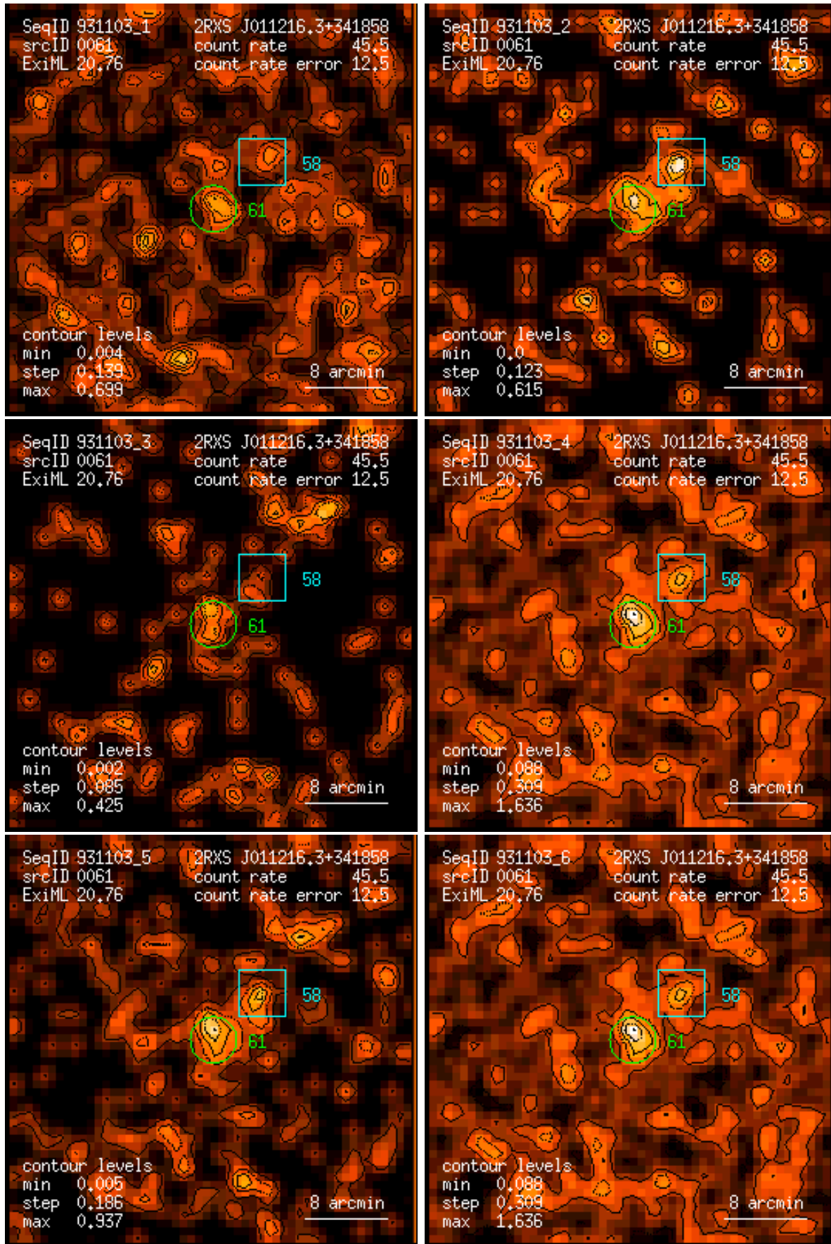
Figure 61: RASS 931103: detection 0061: band rate images, Gaussian filter: (1) PSPC channels 11 – 41, (2) 52 – 90, (3) 91 – 201, (4) 11 – 235, (5) 52 – 201, (6) 11 – 201. Broad band rates in counts/ks. Band rate contour levels in counts/ks/arcmin 2 .
