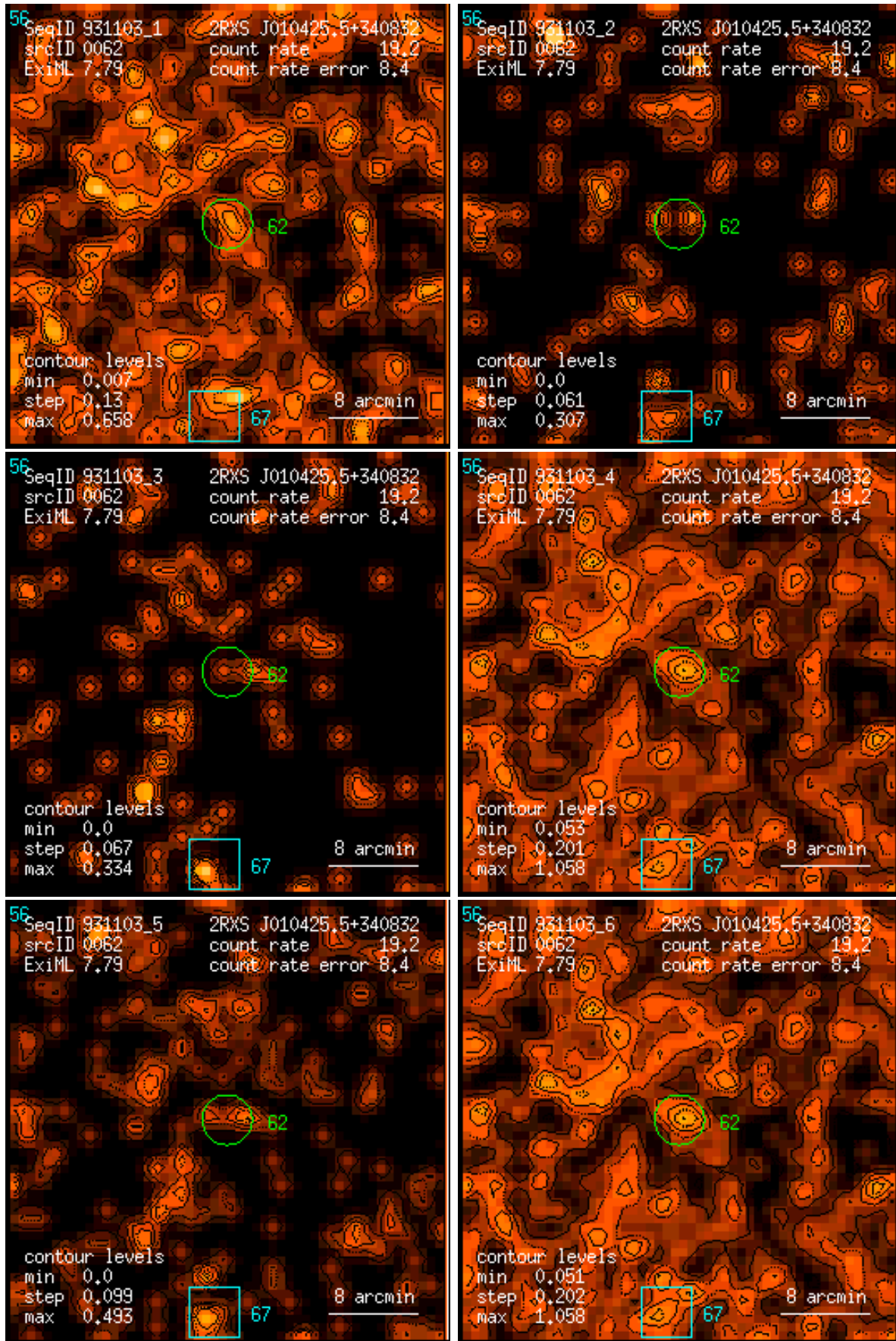
Figure 62: RASS 931103: detection 0062: band rate images, Gaussian filter: (1) PSPC channels 11 – 41, (2) 52 – 90, (3) 91 – 201, (4) 11 – 235, (5) 52 – 201, (6) 11 – 201. Broad band rates in counts/ks. Band rate contour levels in counts/ks/arcmin 2 .
