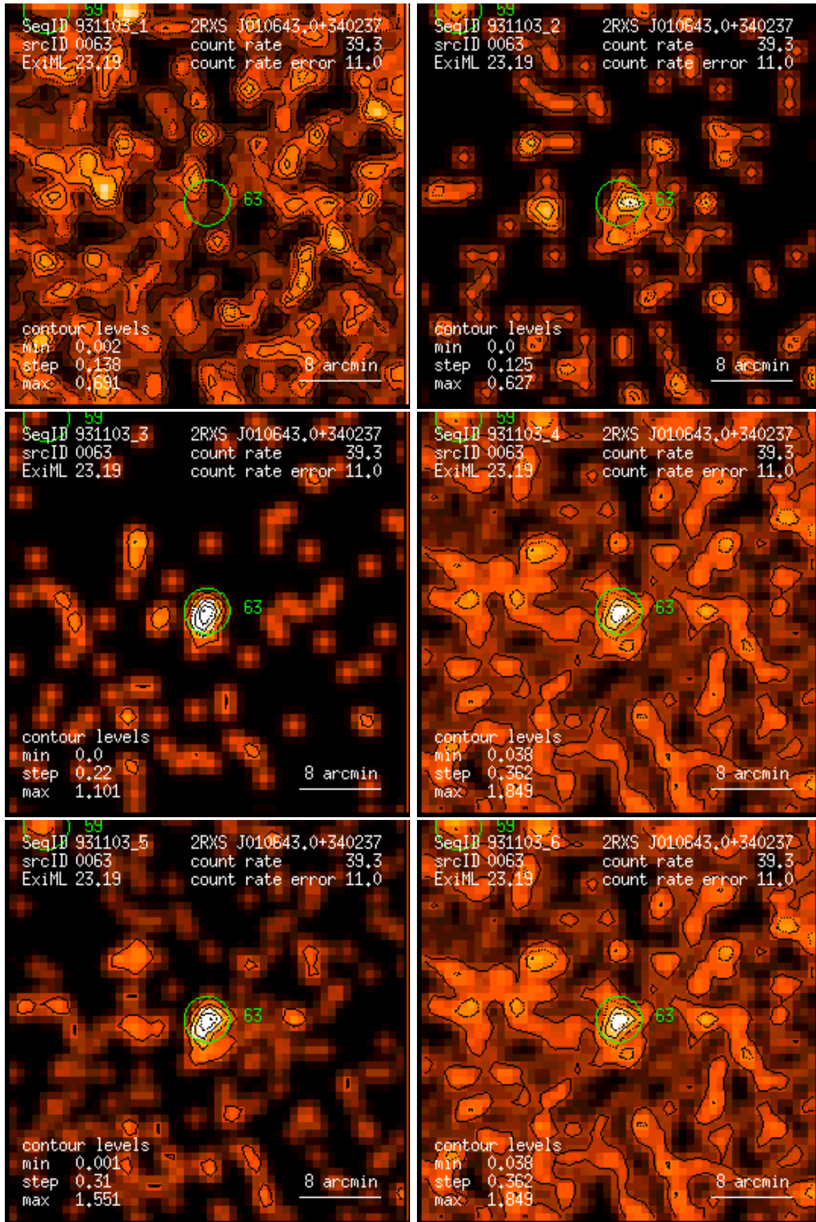
Figure 63: RASS 931103: detection 0063: band rate images, Gaussian filter: (1) PSPC channels 11 – 41, (2) 52 – 90, (3) 91 – 201, (4) 11 – 235, (5) 52 – 201, (6) 11 – 201. Broad band rates in counts/ks. Band rate contour levels in counts/ks/arcmin 2 .
