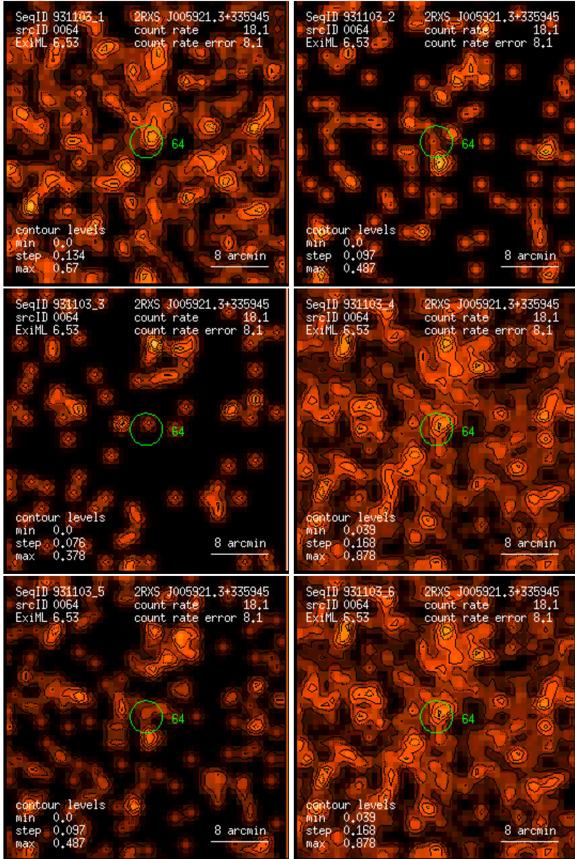
Figure 64: RASS 931103: detection 0064: band rate images, Gaussian filter: (1) PSPC channels 11 – 41, (2) 52 – 90, (3) 91 – 201, (4) 11 – 235, (5) 52 – 201, (6) 11 – 201. Broad band rates in counts/ks. Band rate contour levels in counts/ks/arcmin 2 .
