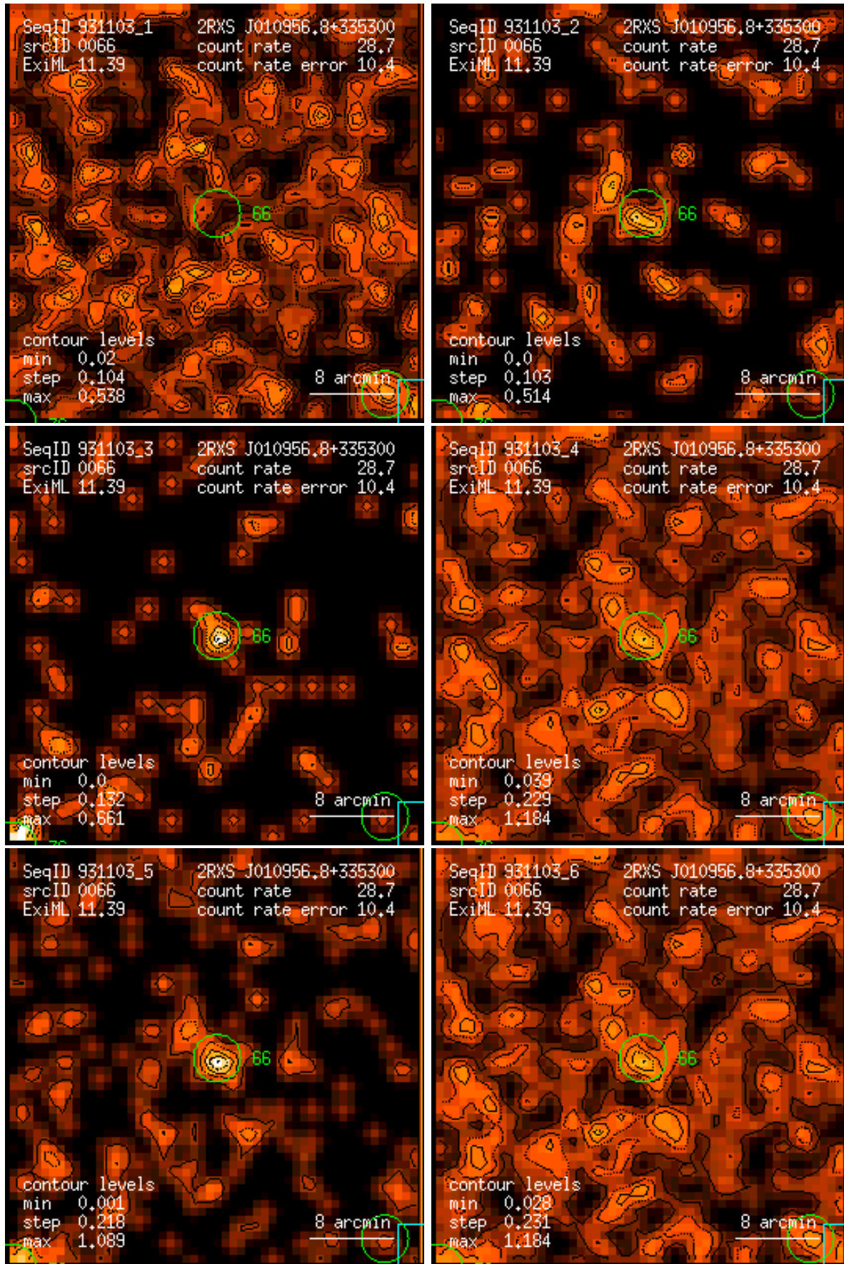
Figure 66: RASS 931103: detection 0066: band rate images, Gaussian filter: (1) PSPC channels 11 – 41, (2) 52 – 90, (3) 91 – 201, (4) 11 – 235, (5) 52 – 201, (6) 11 – 201. Broad band rates in counts/ks. Band rate contour levels in counts/ks/arcmin 2 .
