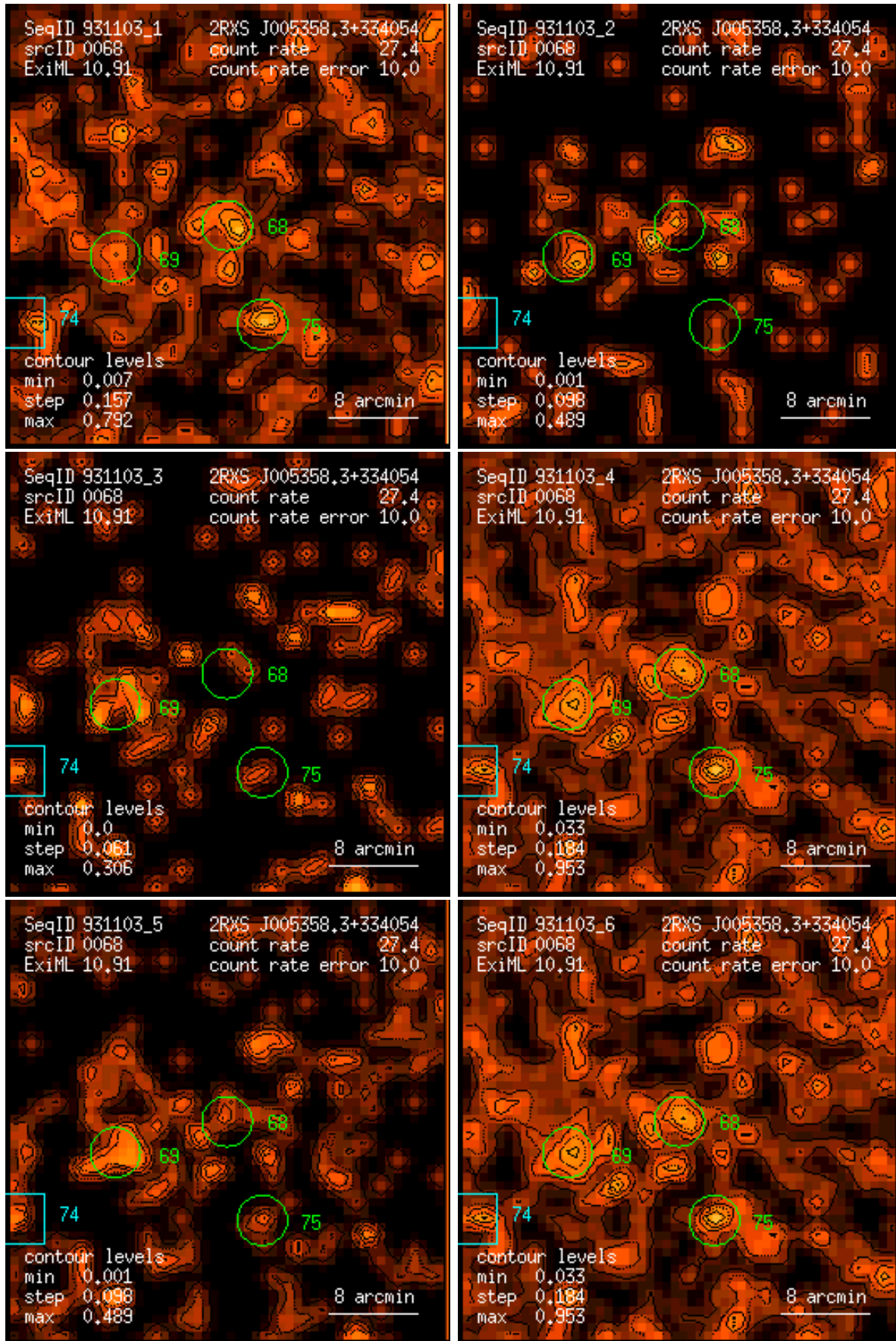
Figure 68: RASS 931103: detection 0068: band rate images, Gaussian filter: (1) PSPC channels 11 – 41, (2) 52 – 90, (3) 91 – 201, (4) 11 – 235, (5) 52 – 201, (6) 11 – 201. Broad band rates in counts/ks. Band rate contour levels in counts/ks/arcmin 2 .
