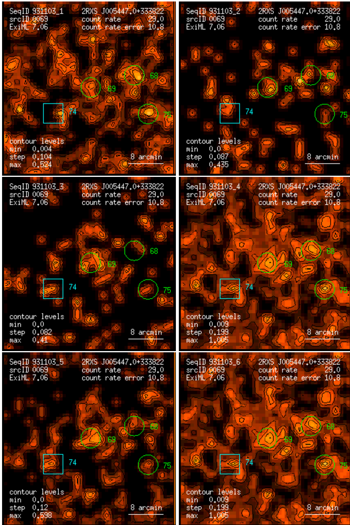
Figure 69: RASS 931103: detection 0069: band rate images, Gaussian filter: (1) PSPC channels 11 – 41, (2) 52 – 90, (3) 91 – 201, (4) 11 – 235, (5) 52 – 201, (6) 11 – 201. Broad band rates in counts/ks. Band rate contour levels in counts/ks/arcmin 2 .
