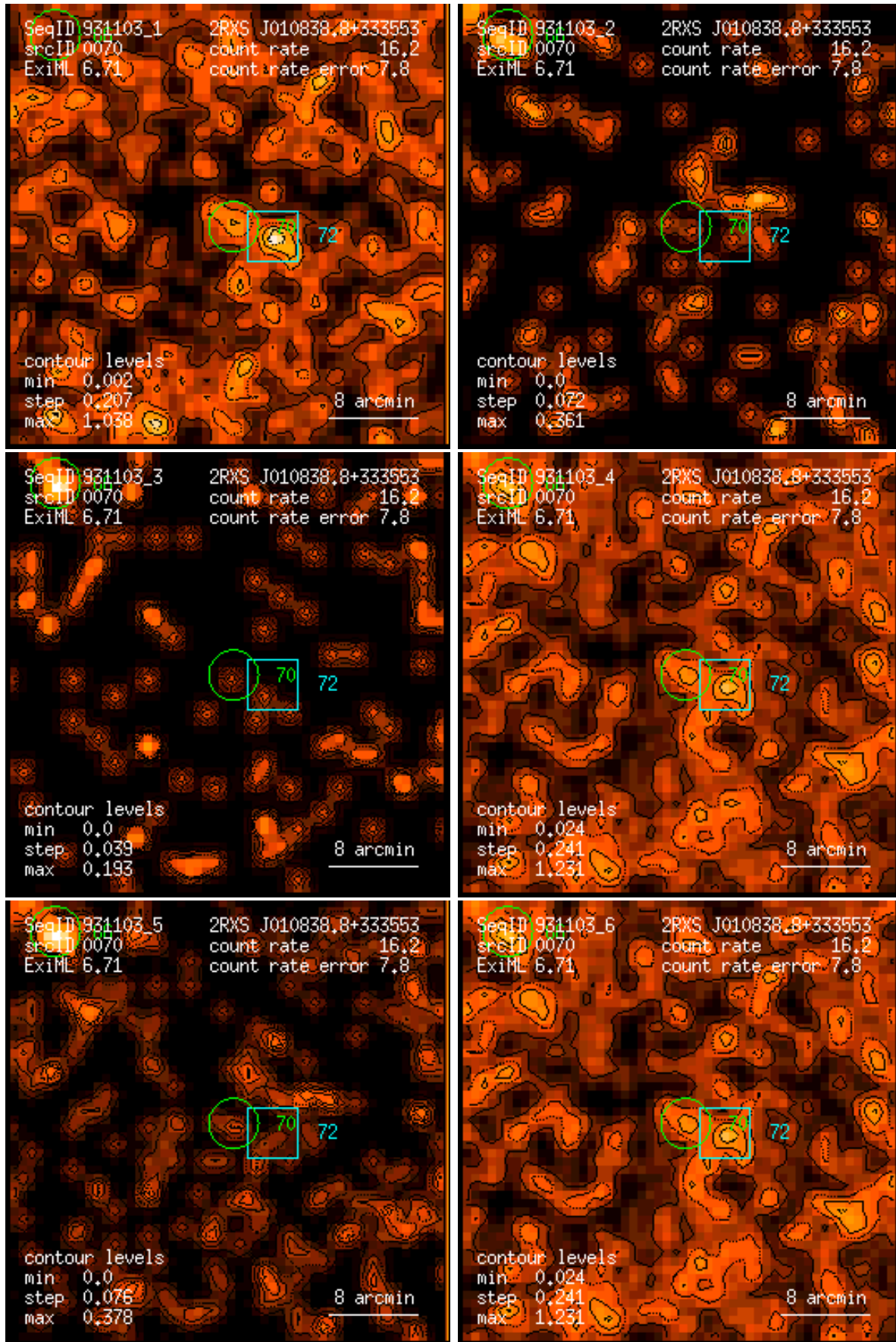
Figure 70: RASS 931103: detection 0070: band rate images, Gaussian filter: (1) PSPC channels 11 – 41, (2) 52 – 90, (3) 91 – 201, (4) 11 – 235, (5) 52 – 201, (6) 11 – 201. Broad band rates in counts/ks. Band rate contour levels in counts/ks/arcmin 2 .
