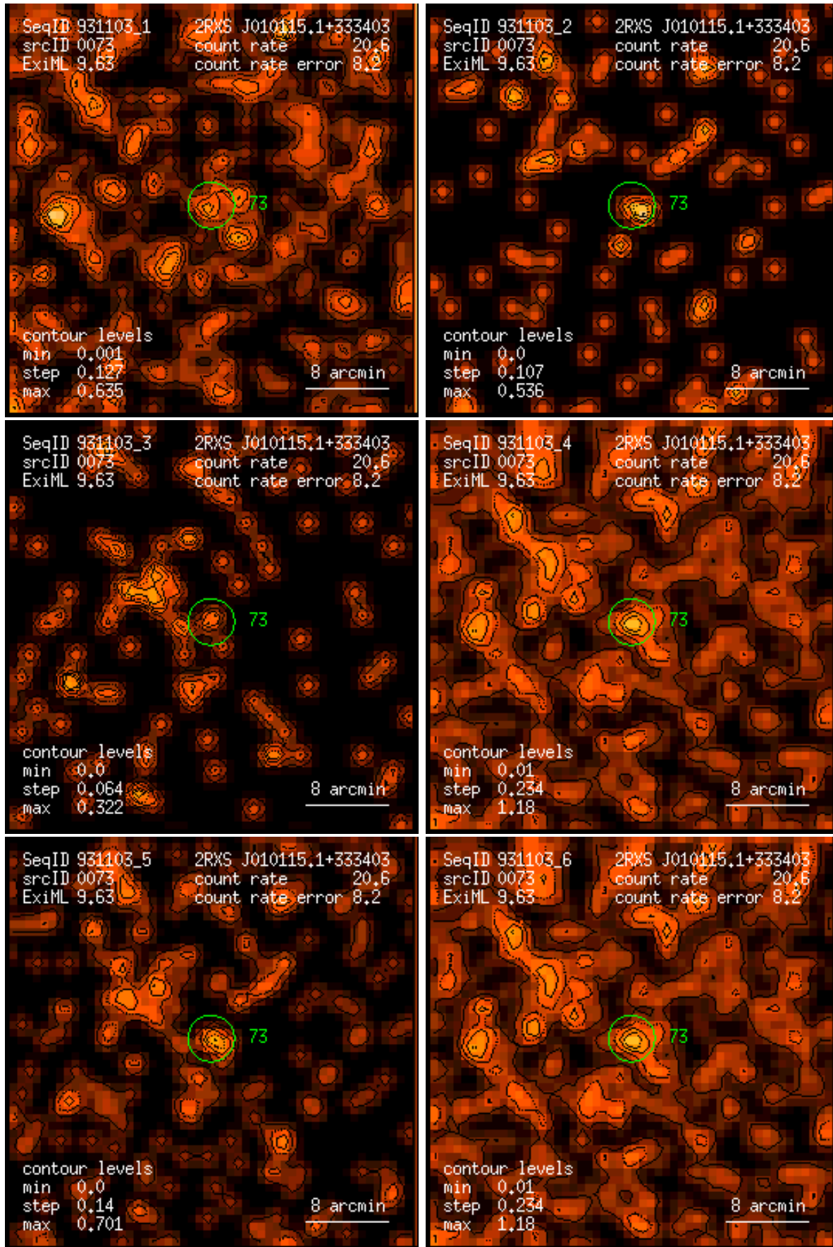
Figure 73: RASS 931103: detection 0073: band rate images, Gaussian filter: (1) PSPC channels 11 – 41, (2) 52 – 90, (3) 91 – 201, (4) 11 – 235, (5) 52 – 201, (6) 11 – 201. Broad band rates in counts/ks. Band rate contour levels in counts/ks/arcmin 2 .
