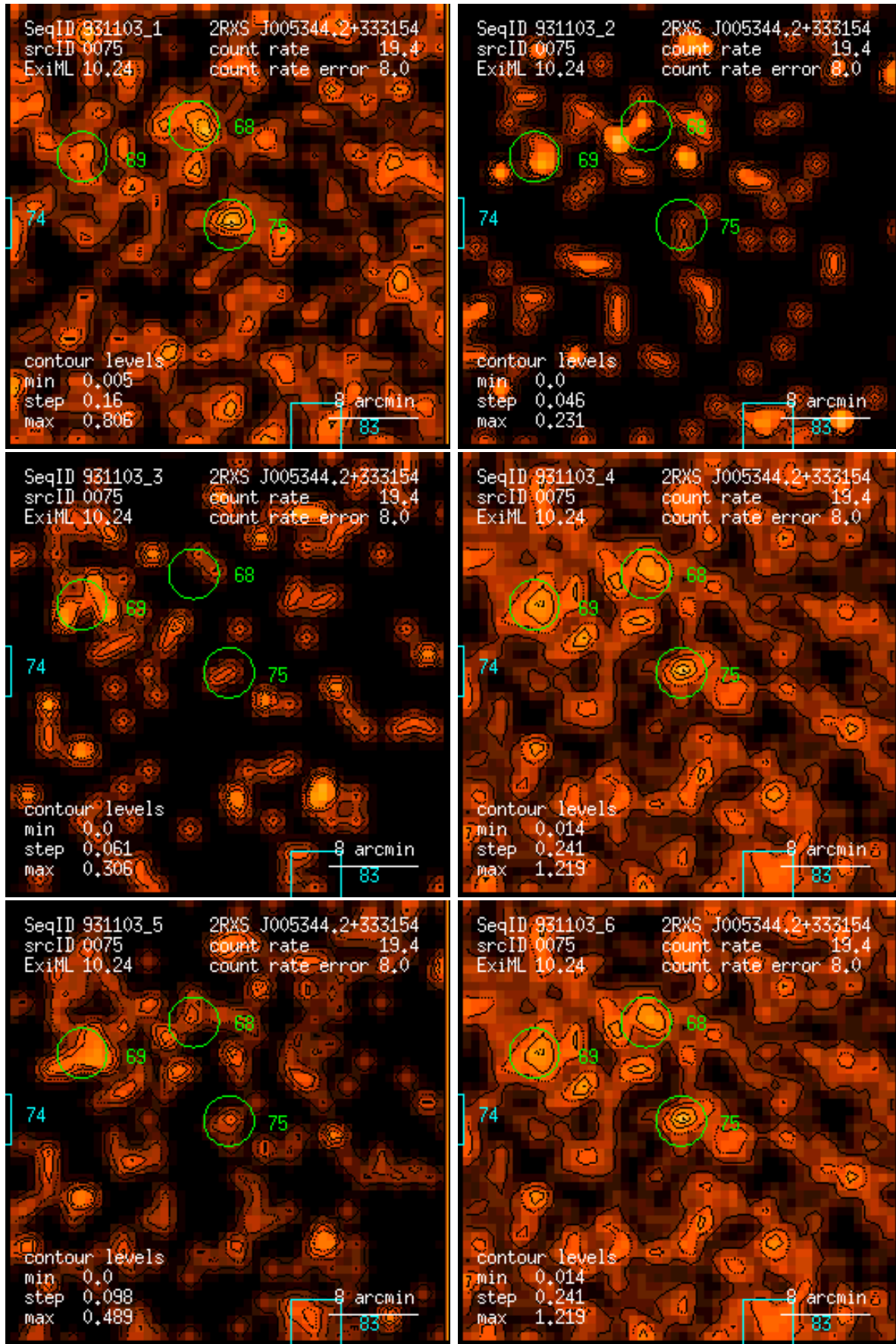
Figure 75: RASS 931103: detection 0075: band rate images, Gaussian filter: (1) PSPC channels 11 – 41, (2) 52 – 90, (3) 91 – 201, (4) 11 – 235, (5) 52 – 201, (6) 11 – 201. Broad band rates in counts/ks. Band rate contour levels in counts/ks/arcmin 2 .
