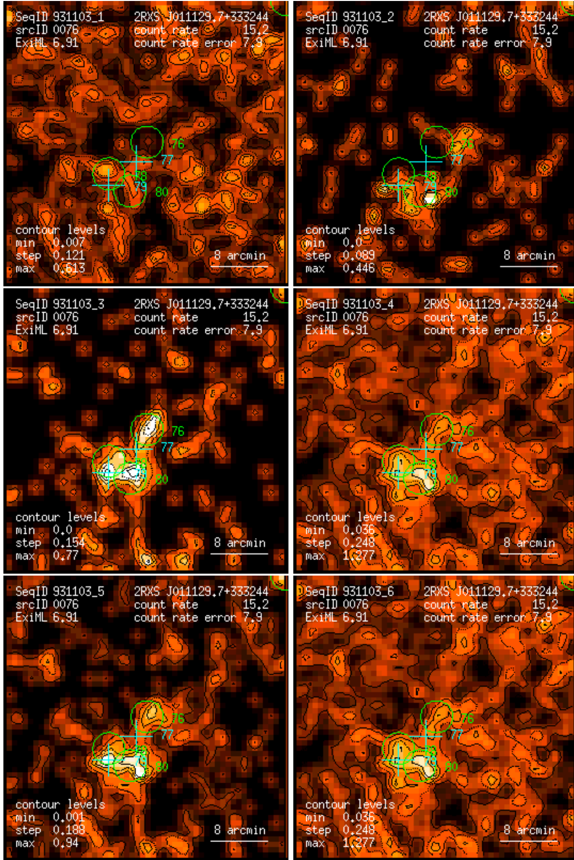
Figure 76: RASS 931103: detection 0076: band rate images, Gaussian filter: (1) PSPC channels 11 – 41, (2) 52 – 90, (3) 91 – 201, (4) 11 – 235, (5) 52 – 201, (6) 11 – 201. Broad band rates in counts/ks. Band rate contour levels in counts/ks/arcmin 2 .
