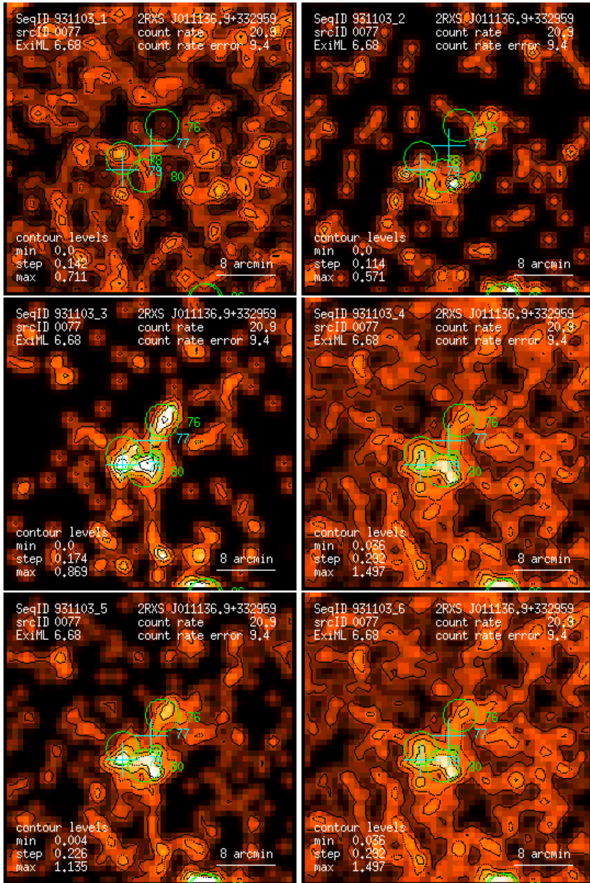
Figure 77: RASS 931103: detection 0077: band rate images, Gaussian filter: (1) PSPC channels 11 – 41, (2) 52 – 90, (3) 91 – 201, (4) 11 – 235, (5) 52 – 201, (6) 11 – 201. Broad band rates in counts/ks. Band rate contour levels in counts/ks/arcmin 2 .
