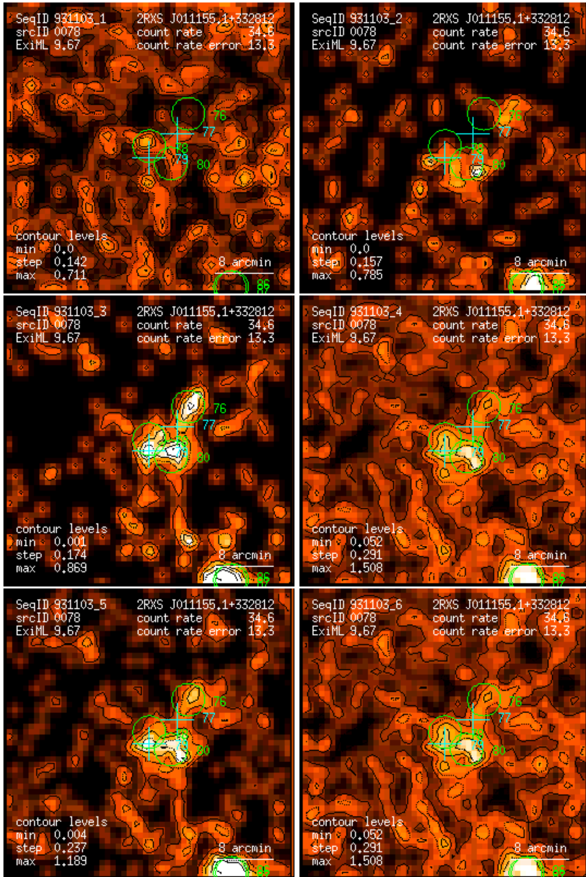
Figure 78: RASS 931103: detection 0078: band rate images, Gaussian filter: (1) PSPC channels 11 – 41, (2) 52 – 90, (3) 91 – 201, (4) 11 – 235, (5) 52 – 201, (6) 11 – 201. Broad band rates in counts/ks. Band rate contour levels in counts/ks/arcmin 2 .
