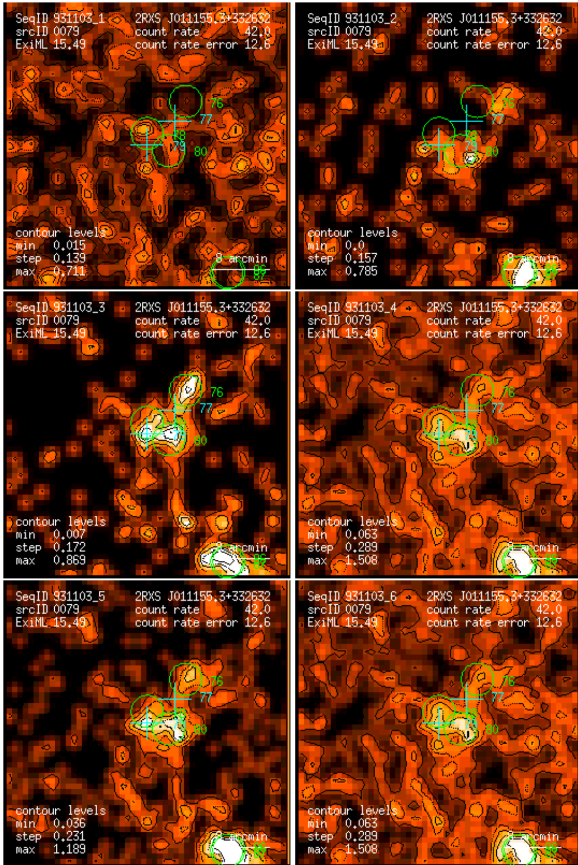
Figure 79: RASS 931103: detection 0079: band rate images, Gaussian filter: (1) PSPC channels 11 – 41, (2) 52 – 90, (3) 91 – 201, (4) 11 – 235, (5) 52 – 201, (6) 11 – 201. Broad band rates in counts/ks. Band rate contour levels in counts/ks/arcmin 2 .
