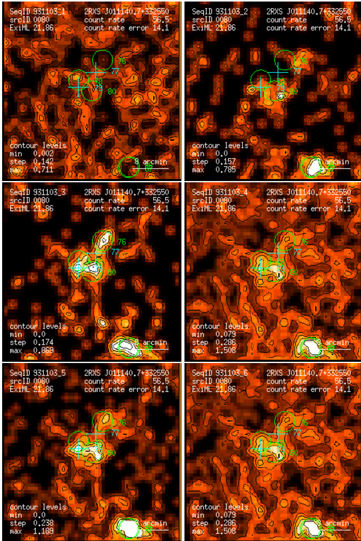
Figure 80: RASS 931103: detection 0080: band rate images, Gaussian filter: (1) PSPC channels 11 – 41, (2) 52 – 90, (3) 91 – 201, (4) 11 – 235, (5) 52 – 201, (6) 11 – 201. Broad band rates in counts/ks. Band rate contour levels in counts/ks/arcmin 2 .
