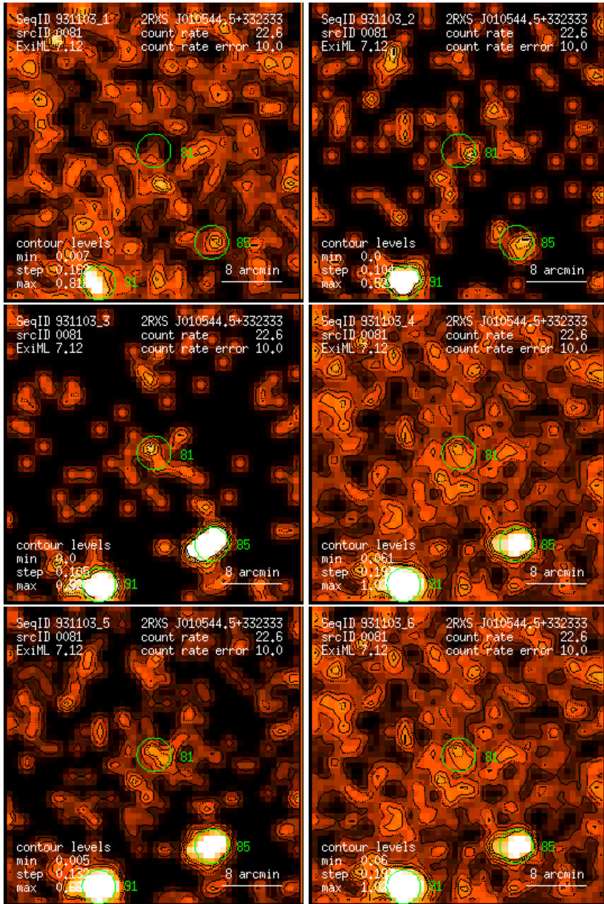
Figure 81: RASS 931103: detection 0081: band rate images, Gaussian filter: (1) PSPC channels 11 – 41, (2) 52 – 90, (3) 91 – 201, (4) 11 – 235, (5) 52 – 201, (6) 11 – 201. Broad band rates in counts/ks. Band rate contour levels in counts/ks/arcmin 2 .
