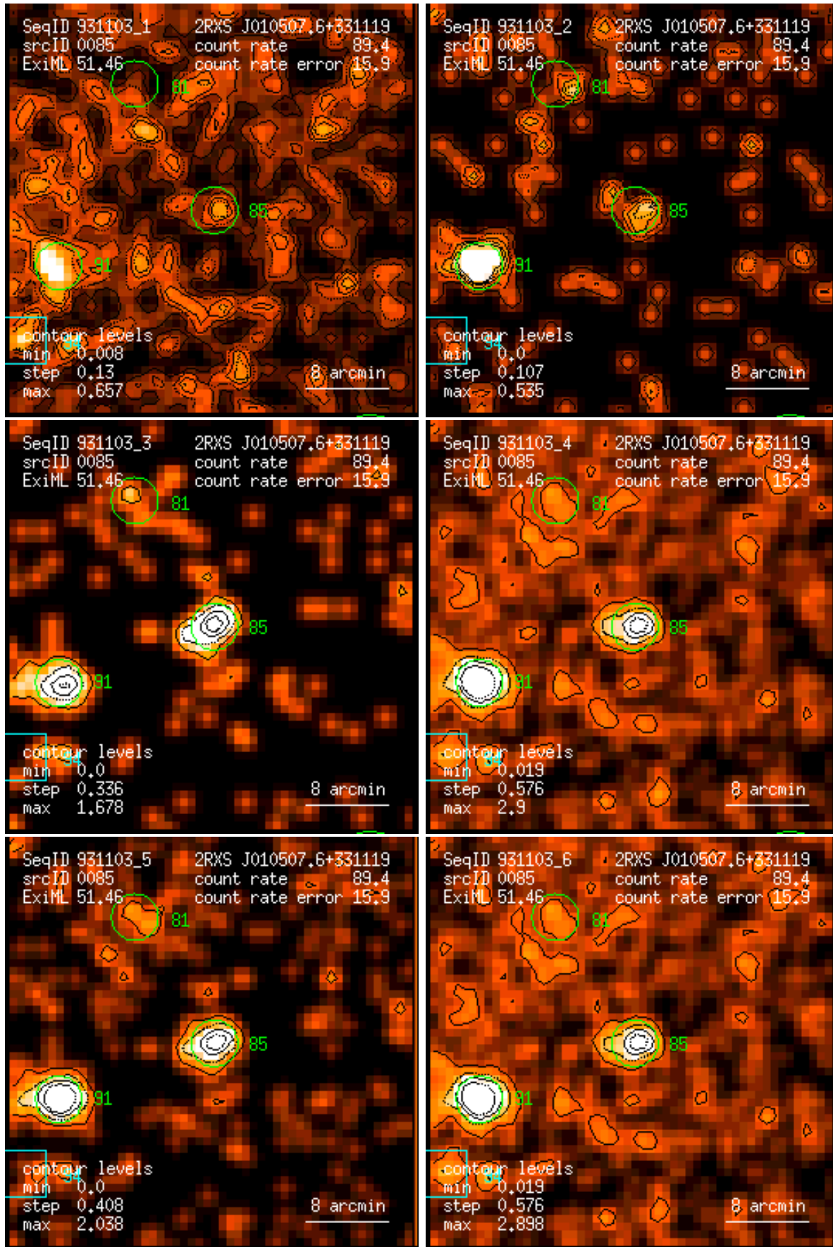
Figure 85: RASS 931103: detection 0085: band rate images, Gaussian filter: (1) PSPC channels 11 – 41, (2) 52 – 90, (3) 91 – 201, (4) 11 – 235, (5) 52 – 201, (6) 11 – 201. Broad band rates in counts/ks. Band rate contour levels in counts/ks/arcmin 2 .
