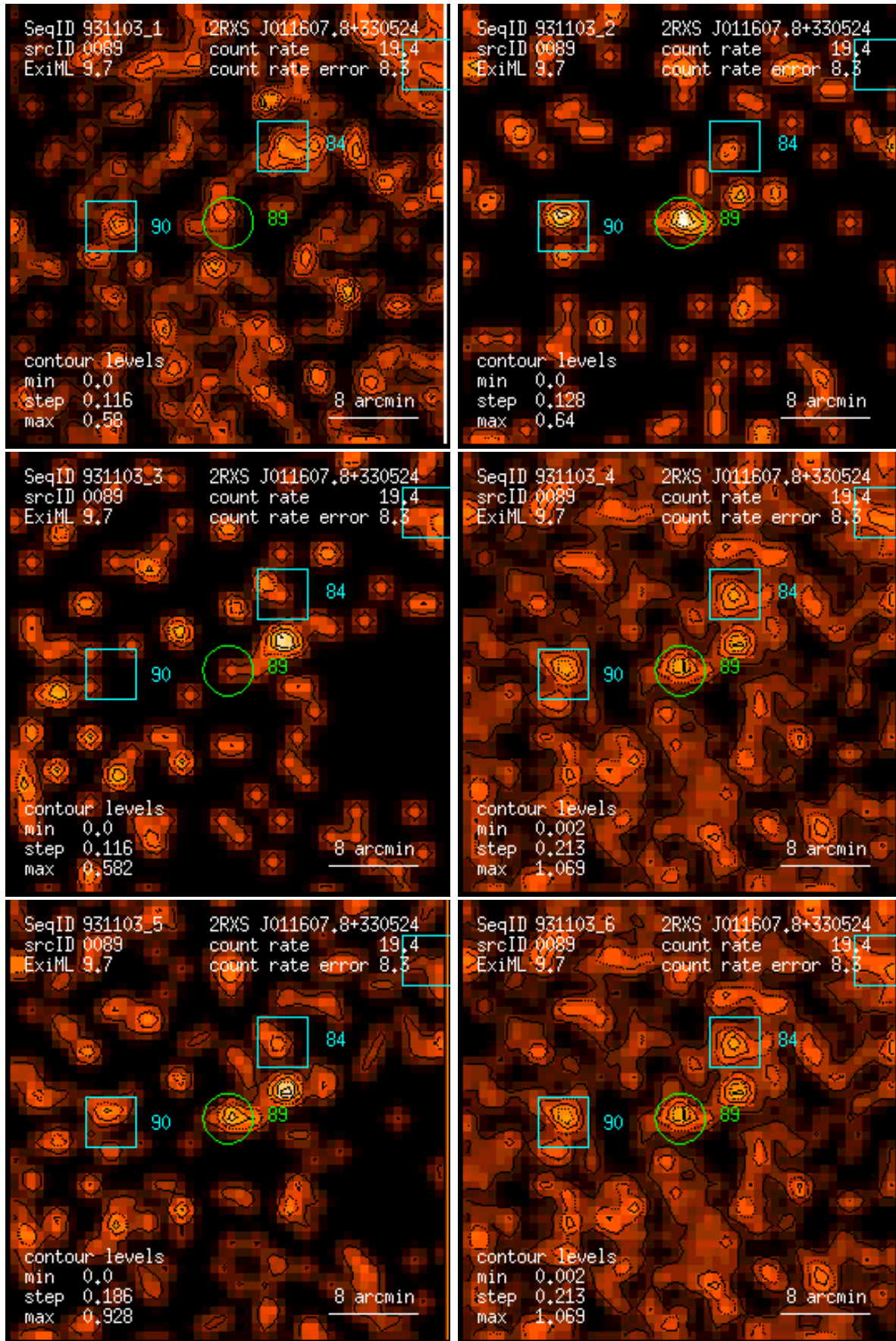
Figure 89: RASS 931103: detection 0089: band rate images, Gaussian filter: (1) PSPC channels 11 – 41, (2) 52 – 90, (3) 91 – 201, (4) 11 – 235, (5) 52 – 201, (6) 11 – 201. Broad band rates in counts/ks. Band rate contour levels in counts/ks/arcmin 2 .
