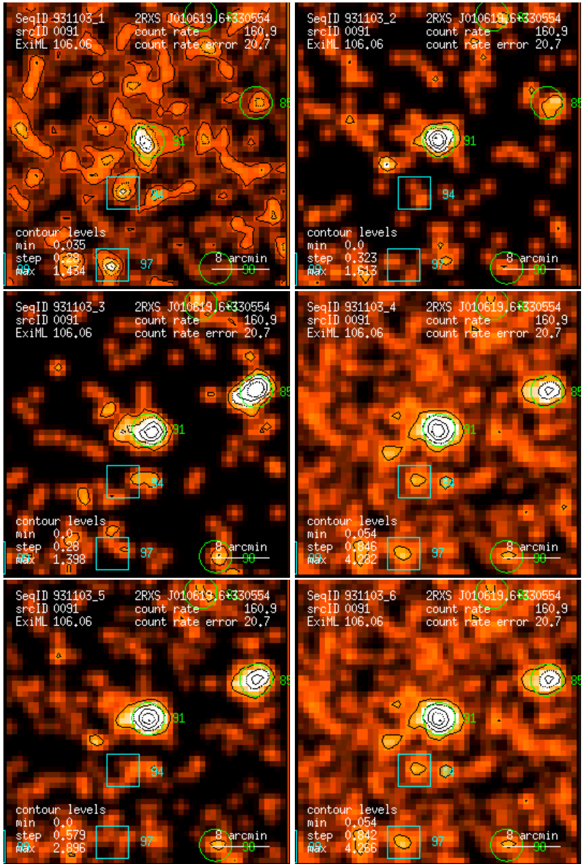
Figure 91: RASS 931103: detection 0091: band rate images, Gaussian filter: (1) PSPC channels 11 – 41, (2) 52 – 90, (3) 91 – 201, (4) 11 – 235, (5) 52 – 201, (6) 11 – 201. Broad band rates in counts/ks. Band rate contour levels in counts/ks/arcmin 2 .
