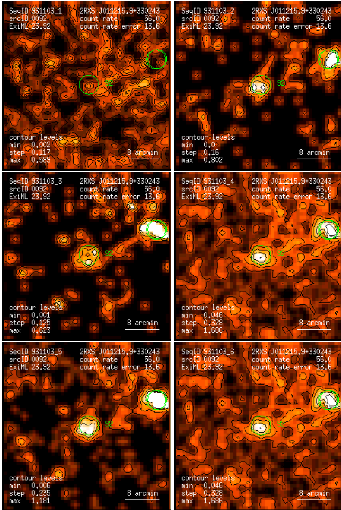
Figure 92: RASS 931103: detection 0092: band rate images, Gaussian filter: (1) PSPC channels 11 – 41, (2) 52 – 90, (3) 91 – 201, (4) 11 – 235, (5) 52 – 201, (6) 11 – 201. Broad band rates in counts/ks. Band rate contour levels in counts/ks/arcmin 2 .
