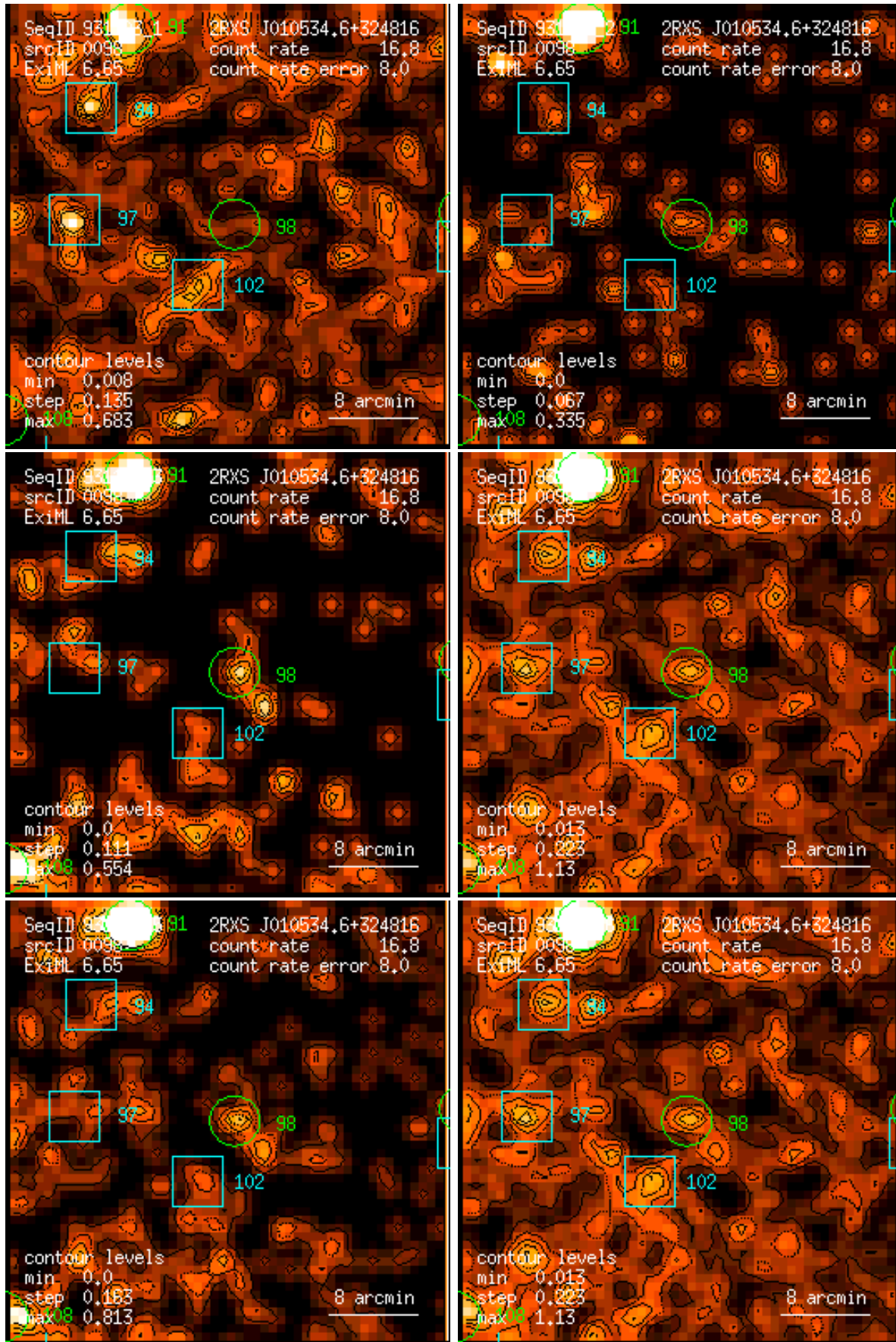
Figure 98: RASS 931103: detection 0098: band rate images, Gaussian filter: (1) PSPC channels 11 – 41, (2) 52 – 90, (3) 91 – 201, (4) 11 – 235, (5) 52 – 201, (6) 11 – 201. Broad band rates in counts/ks. Band rate contour levels in counts/ks/arcmin 2 .
