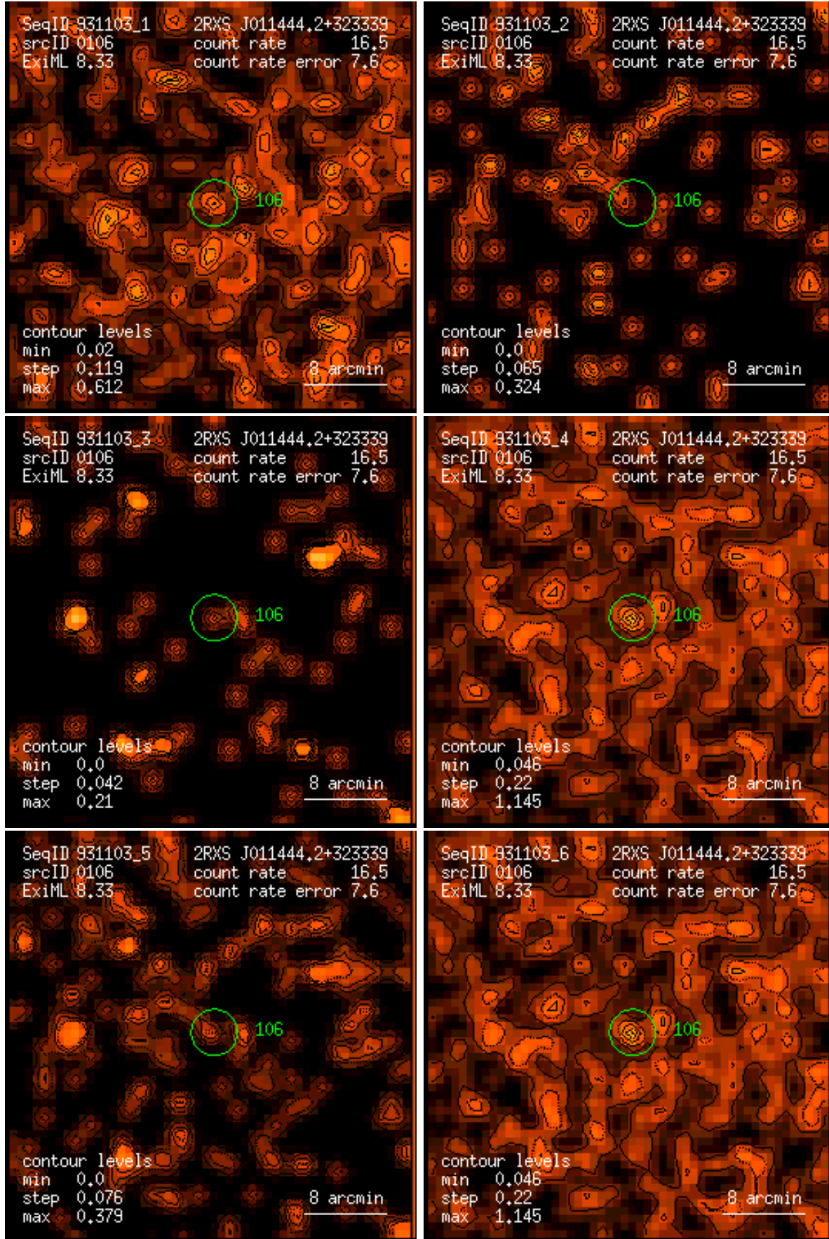
Figure 106: RASS 931103: detection 0106: band rate images, Gaussian filter: (1) PSPC channels 11 – 41, (2) 52 – 90, (3) 91 – 201, (4) 11 – 235, (5) 52 – 201, (6) 11 – 201. Broad band rates in counts/ks. Band rate contour levels in counts/ks/arcmin 2 .
