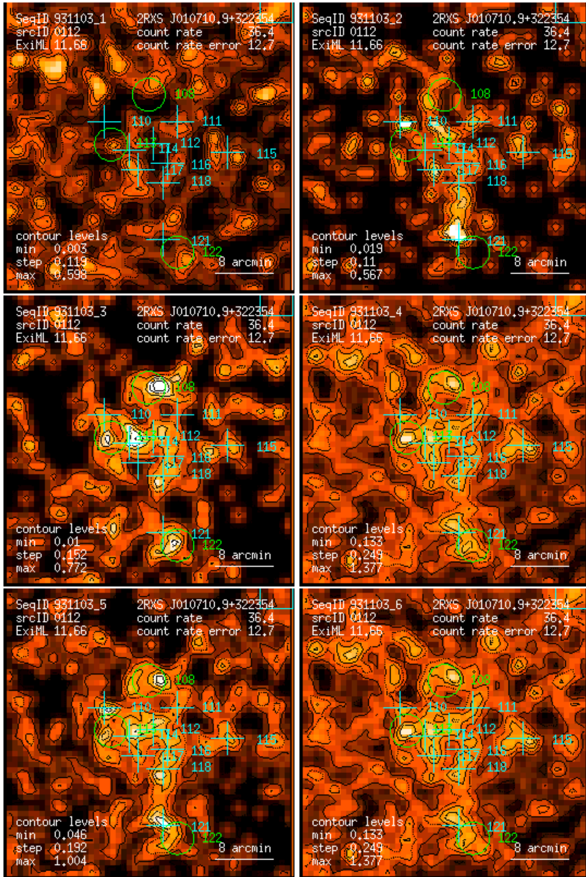
Figure 112: RASS 931103: detection 0112: band rate images, Gaussian filter: (1) PSPC channels 11 – 41, (2) 52 – 90, (3) 91 – 201, (4) 11 – 235, (5) 52 – 201, (6) 11 – 201. Broad band rates in counts/ks. Band rate contour levels in counts/ks/arcmin 2 .
