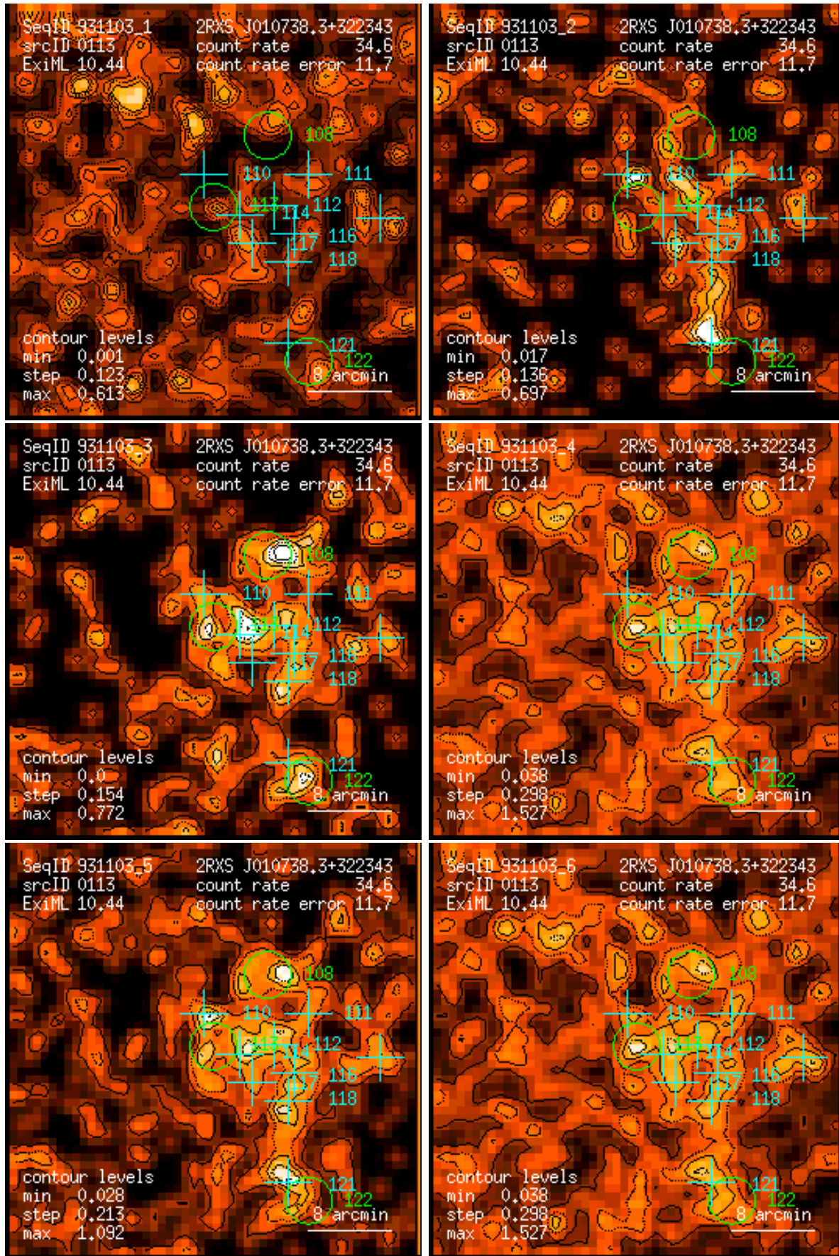
Figure 113: RASS 931103: detection 0113: band rate images, Gaussian filter: (1) PSPC channels 11 – 41, (2) 52 – 90, (3) 91 – 201, (4) 11 – 235, (5) 52 – 201, (6) 11 – 201. Broad band rates in counts/ks. Band rate contour levels in counts/ks/arcmin 2 .
