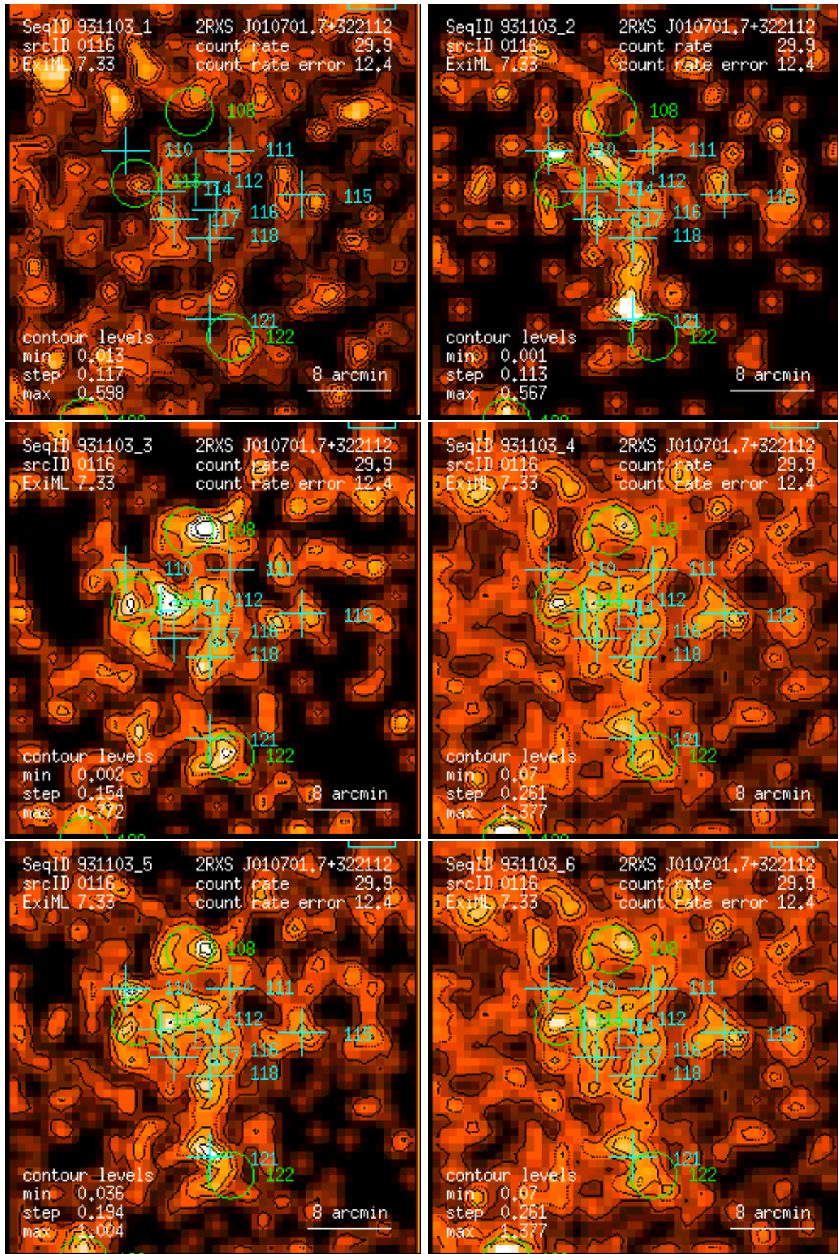
Figure 116: RASS 931103: detection 0116: band rate images, Gaussian filter: (1) PSPC channels 11 – 41, (2) 52 – 90, (3) 91 – 201, (4) 11 – 235, (5) 52 – 201, (6) 11 – 201. Broad band rates in counts/ks. Band rate contour levels in counts/ks/arcmin 2 .
