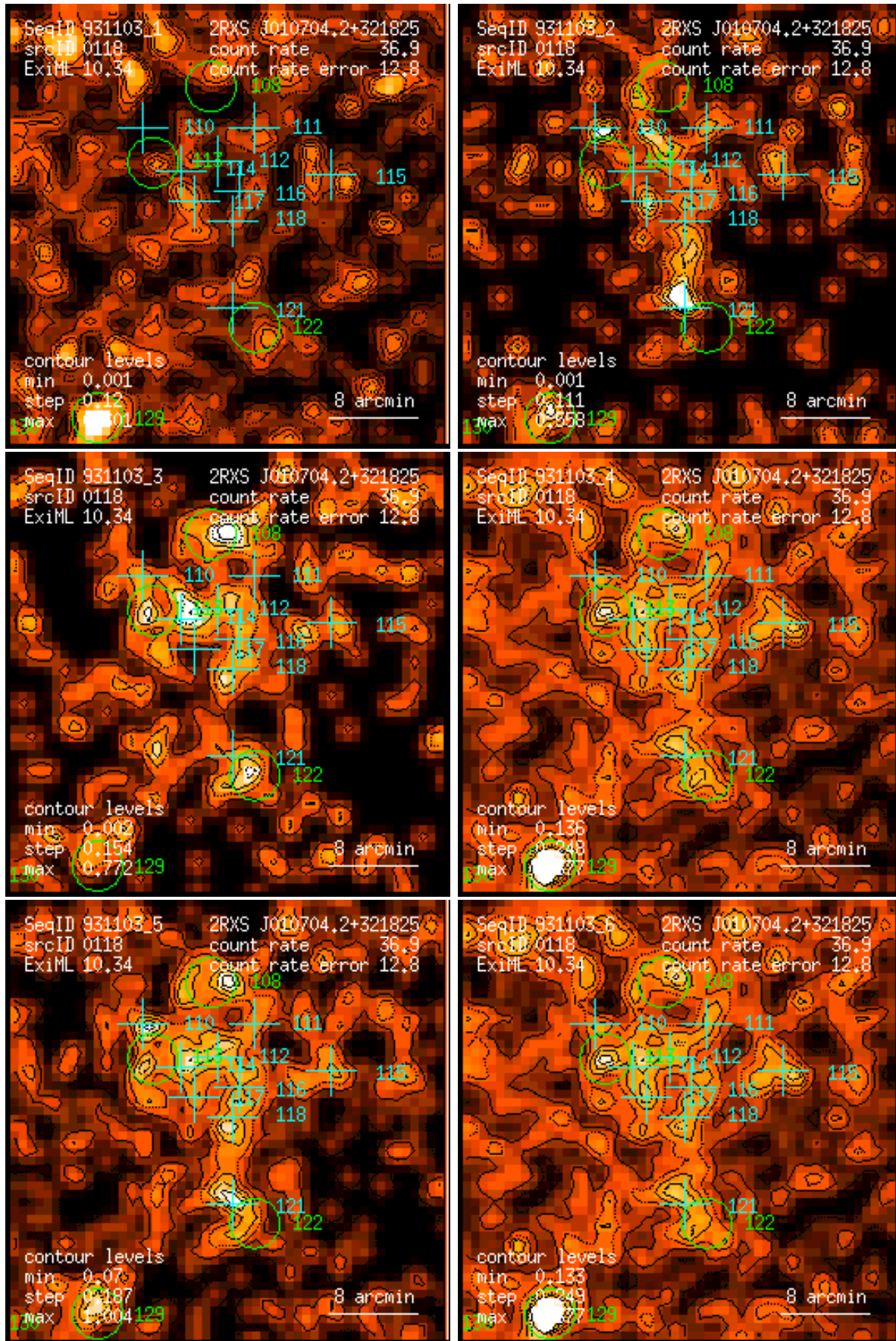
Figure 118: RASS 931103: detection 0118: band rate images, Gaussian filter: (1) PSPC channels 11 – 41, (2) 52 – 90, (3) 91 – 201, (4) 11 – 235, (5) 52 – 201, (6) 11 – 201. Broad band rates in counts/ks. Band rate contour levels in counts/ks/arcmin 2 .
