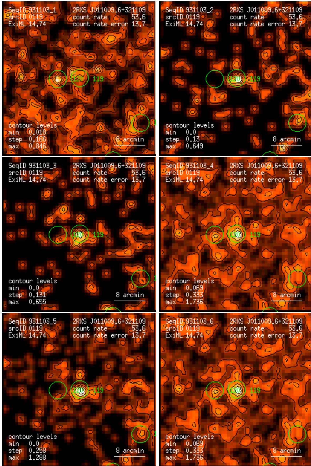
Figure 119: RASS 931103: detection 0119: band rate images, Gaussian filter: (1) PSPC channels 11 – 41, (2) 52 – 90, (3) 91 – 201, (4) 11 – 235, (5) 52 – 201, (6) 11 – 201. Broad band rates in counts/ks. Band rate contour levels in counts/ks/arcmin 2 .
