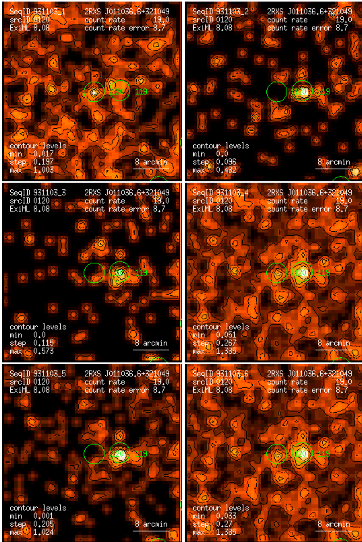
Figure 120: RASS 931103: detection 0120: band rate images, Gaussian filter: (1) PSPC channels 11 – 41, (2) 52 – 90, (3) 91 – 201, (4) 11 – 235, (5) 52 – 201, (6) 11 – 201. Broad band rates in counts/ks. Band rate contour levels in counts/ks/arcmin 2 .
