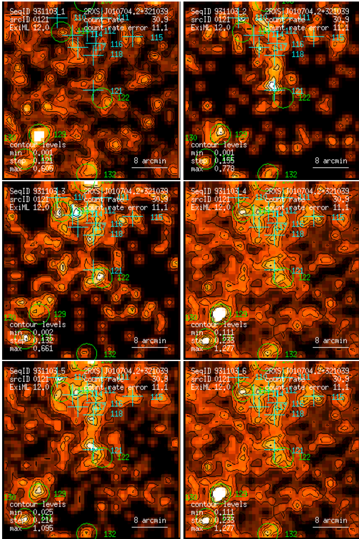
Figure 121: RASS 931103: detection 0121: band rate images, Gaussian filter: (1) PSPC channels 11 – 41, (2) 52 – 90, (3) 91 – 201, (4) 11 – 235, (5) 52 – 201, (6) 11 – 201. Broad band rates in counts/ks. Band rate contour levels in counts/ks/arcmin 2 .
