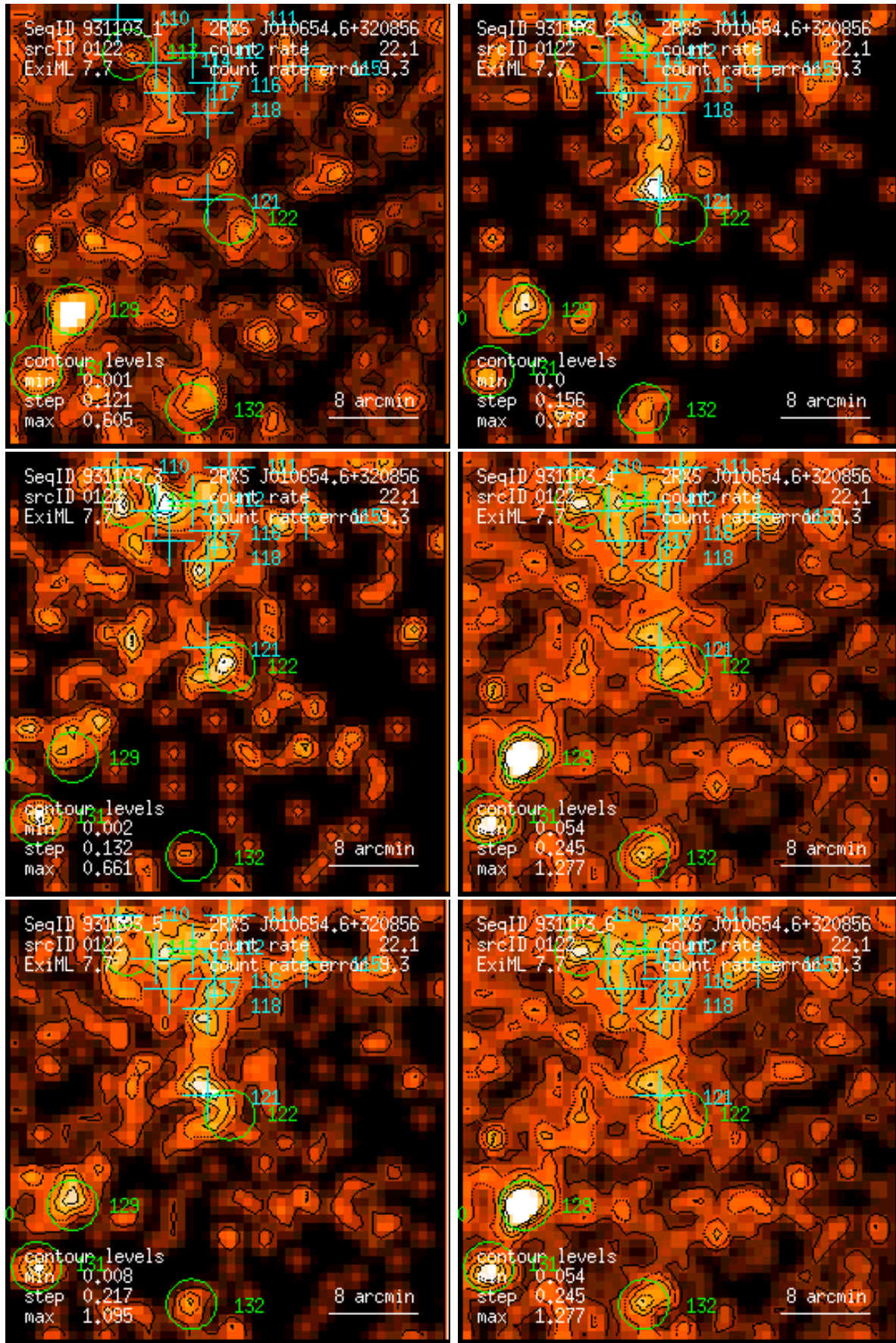
Figure 122: RASS 931103: detection 0122: band rate images, Gaussian filter: (1) PSPC channels 11 – 41, (2) 52 – 90, (3) 91 – 201, (4) 11 – 235, (5) 52 – 201, (6) 11 – 201. Broad band rates in counts/ks. Band rate contour levels in counts/ks/arcmin 2 .
